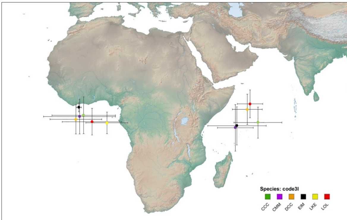
Figure 17: Latitudinal and longitudinal barycentres and standard deviations of each marine turtle species observed by observers around a floating device in the Atlantic and Indian
