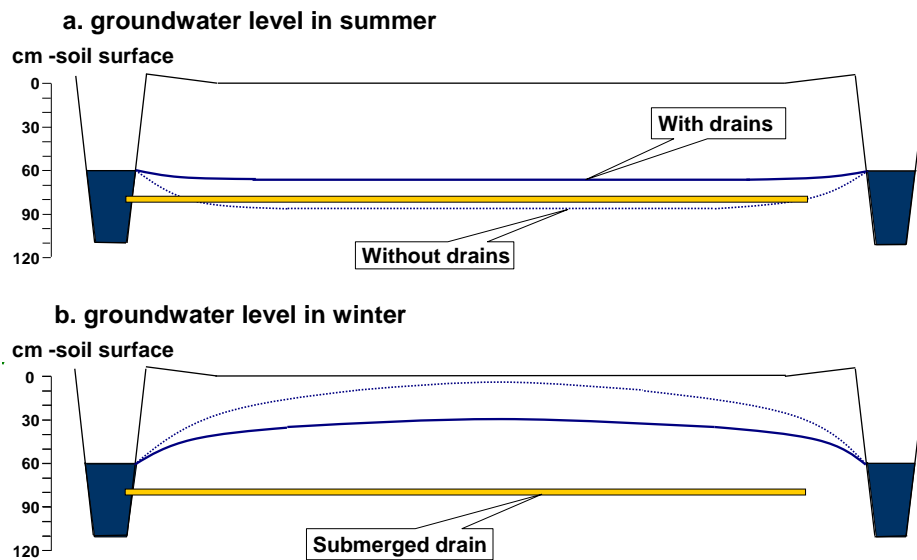
Fig. 1: Reduction of peat oxidation and subsidence and CO 2 -emissions by raising groundwater levels with infiltration via submerged drains in summer level. In wet periods the submerged drains will function as drainage.
