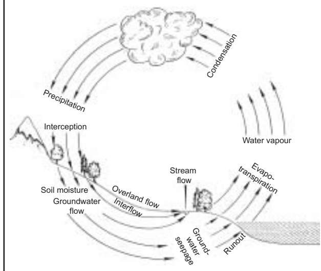
FIGURE 2 Simplified diagram of the hydrological cycle (Adapted from Ward, 1975)
