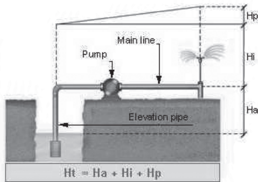
FIGURE 3.51 - Ht is the total head, Ha is the elevation head, Hi is the emitter operation head and Hp is the friction losses head (sum of friction losses in the main line, submain, manifolds, laterals, valves, pipe fittings and minor losses).
