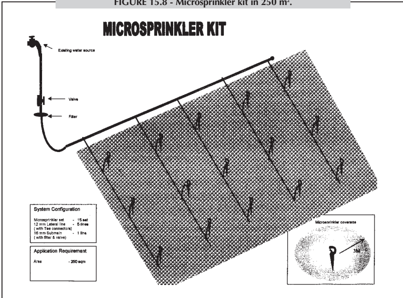
FIGURE 15.8 - Microsprinkler kit in 250 m 2 .
