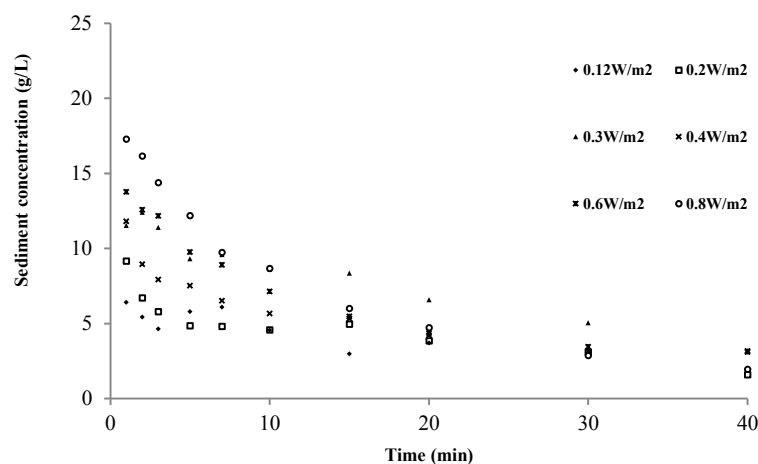
Figure 1: Dynamic changes of sediment concentration at different streampowers for the marl sample.
