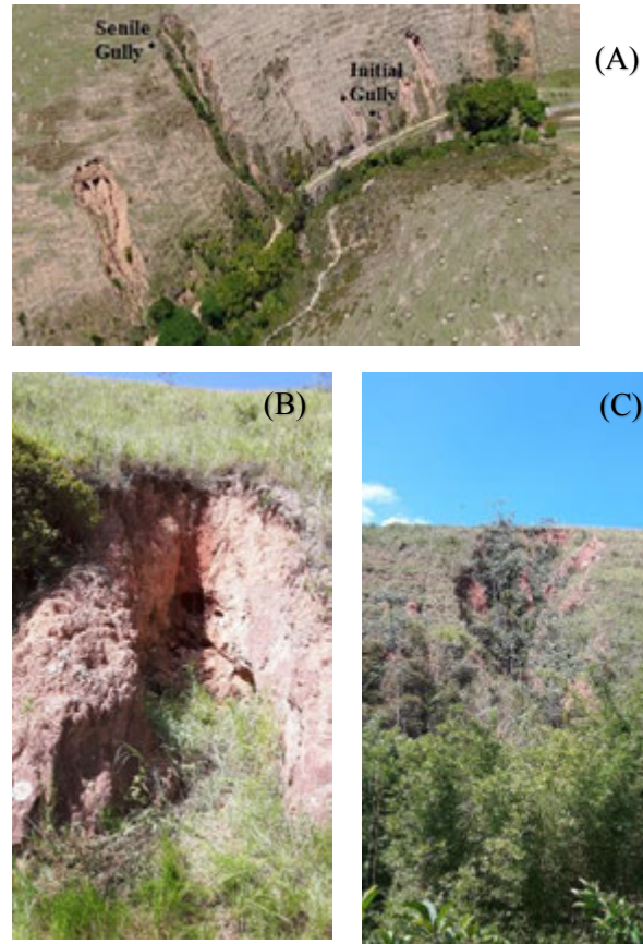
Figure 1: Morphological classification of two gullies in different evolutionary stages, initial (B) and senile (C), Pinheiral municipality, Rio de Janeiro State.
