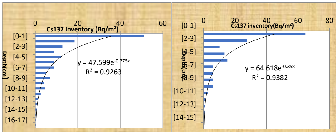
Figure 2: 137 Cs profile distribution in reference site
