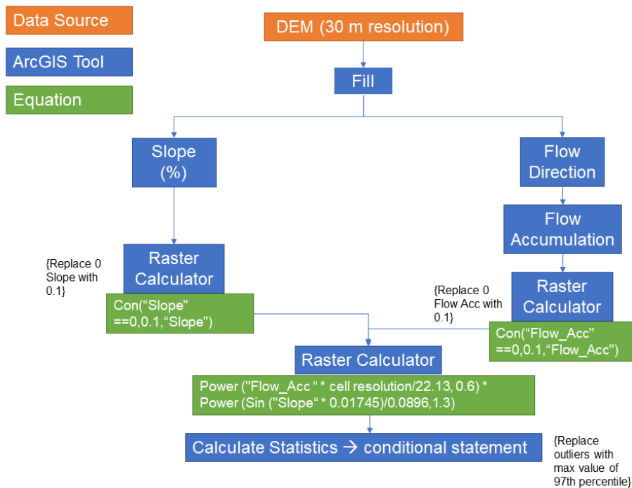
Figure 2: Flowchart for calculating the LS factor
