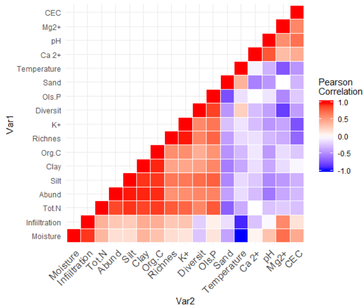
Figure 1: Relationships between termites’ composition and soil properties across the restored sites. Nb: correlation coefficient of 0.60–0.79 is significant, and from 0.80 to 1 is very significant.
