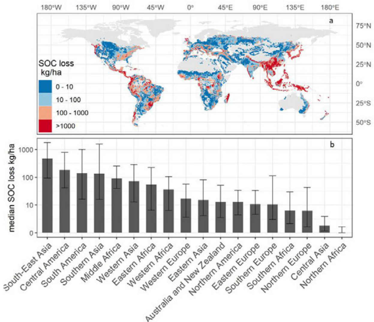
Figure 1: Simulated annual loss of SOC in sediment runoff of maize fields (1980 – 2010) in the baseline tillage scenario "MIX". a: Annual loss of SOC simulated for more than 100 000 grids, where daily growth of maize and water erosion is simulated. b: Median and error bars with first quartiles and third quartiles of simulated annual SOC loss in sediments for major world regions.
