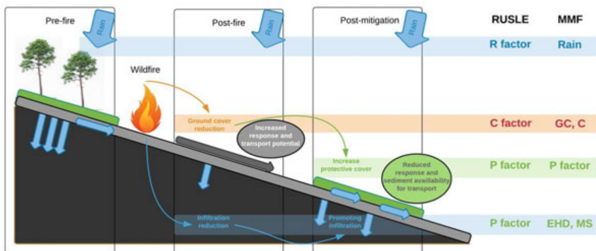
Figure 1: Post-fire runoff-erosion processes and their parameterization in the RUSLE and MMF models (adapted from Vieira et al. , 2018).
