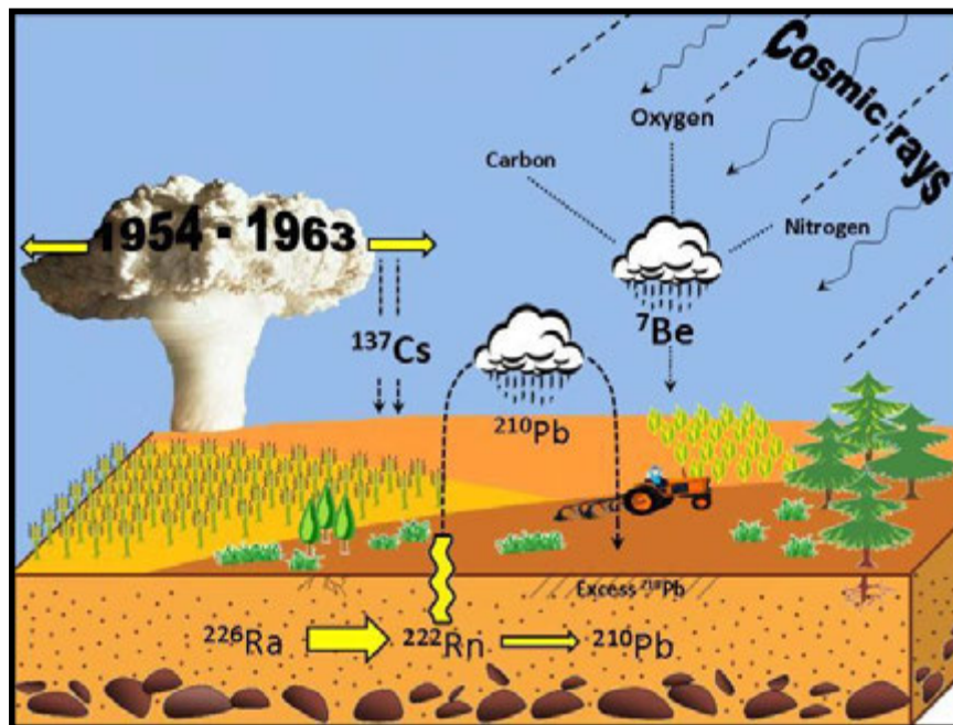
Figure 1: Radiogenic isotopes being used for assessing on-site soil erosion rates. Adapted from Zupanc & Mabit, 2010 – Dela, 33, 21–36.
