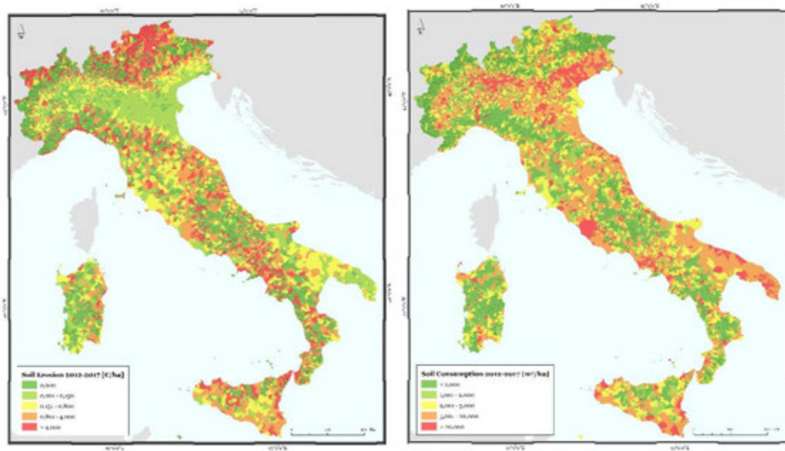
Figure 1: Loss of erosion control produced by land consumption between 2012 and 2017 - maximum value per Municipality \text{€} \cdot \text{y}^{-1}
