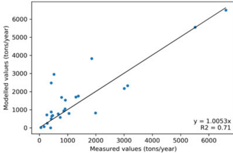
Figure 1: Relationship between measured and modelled sediment loads (tons/year) for 26 catchments in Flanders (Deproost et al. , 2018)
