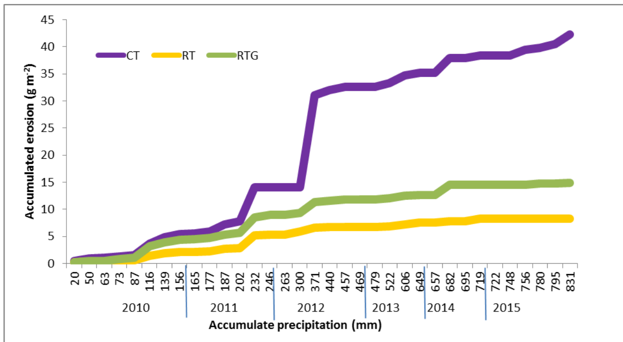
Figure 2: Accumulated erosion versus accumulated precipitation during the study period in the wheat (above) and almond (below) fields.
