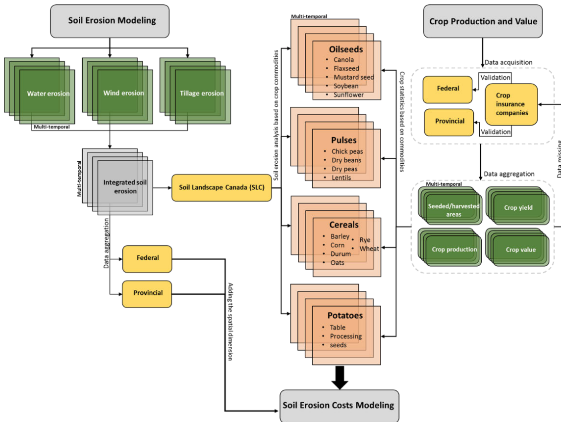
Figure 1: Illustration of the soil erosion costs analysis for crop commodities in Canada for the period between 1961 and 2016.
