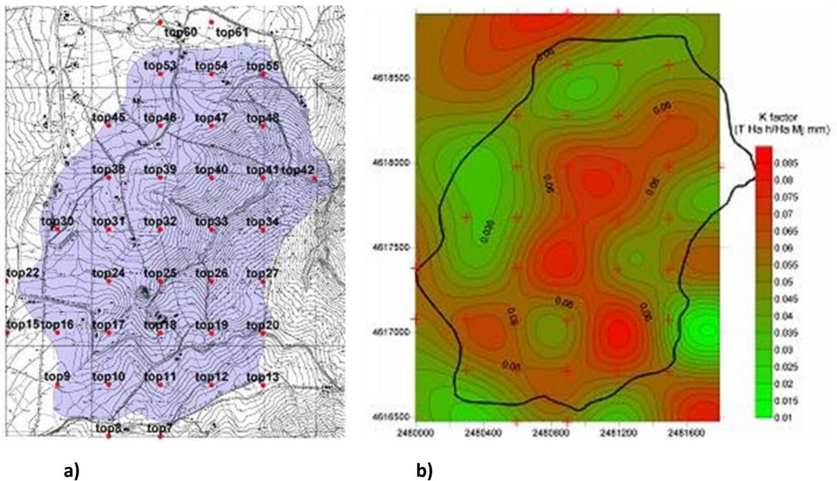
Figure 2: a) Location of topsoil samples within the test area; b) spatial interpolation of the K factor calculated by the formula of Wischmeier and Smith (1978).
