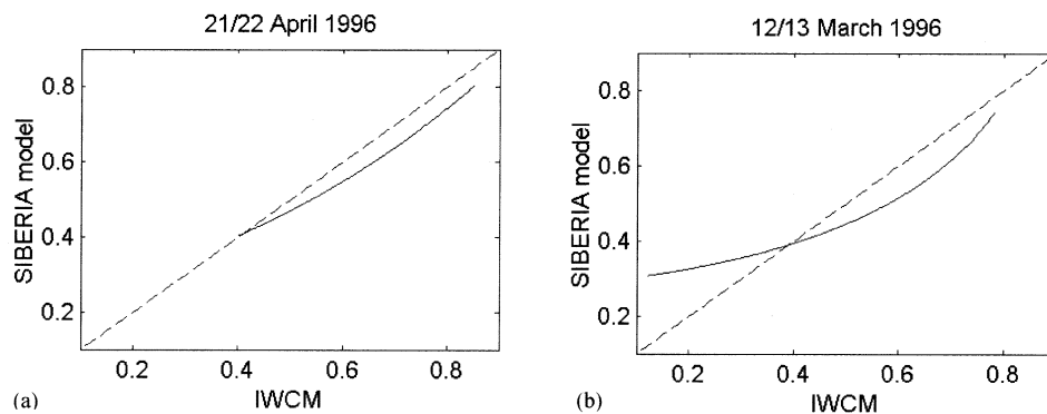
Fig. 4. Illustrating values for coherence as derived from IWCM and from model used in the SIBERIA project. (a) Short baseline case ( B_n = 55 m). (b) Long baseline case ( B_n = 218 m).
