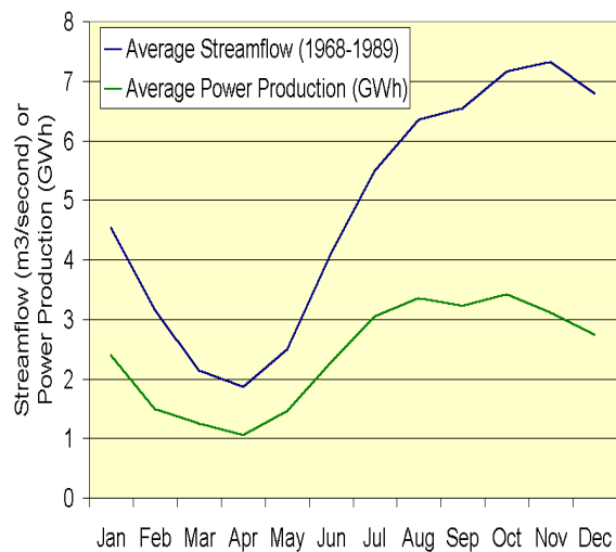
Figure 2: Average annual hydrograph of La Esperanza River & energy production at LEHP. Bel Ing., 1994.
