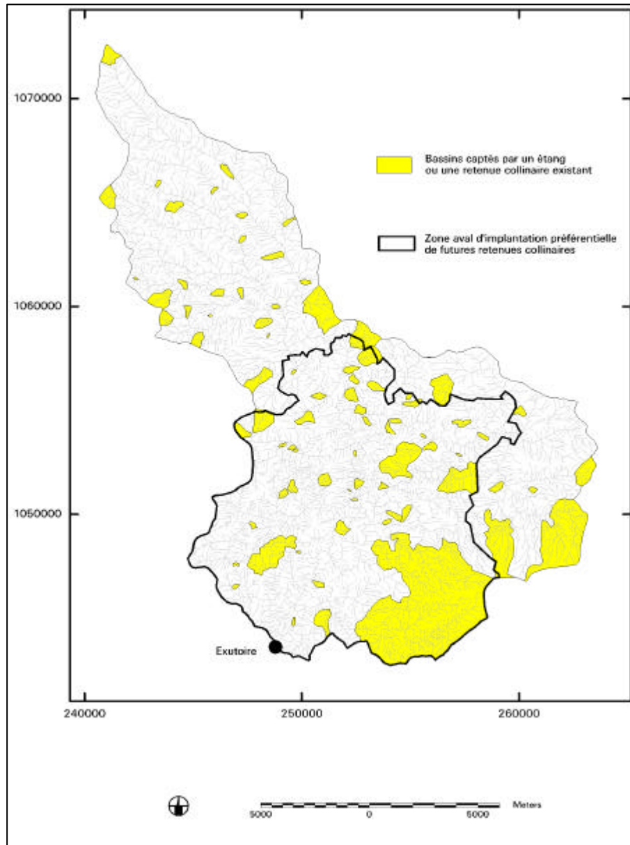
FIGURE 1 The Yvel watershed (Lambert geographical system)
