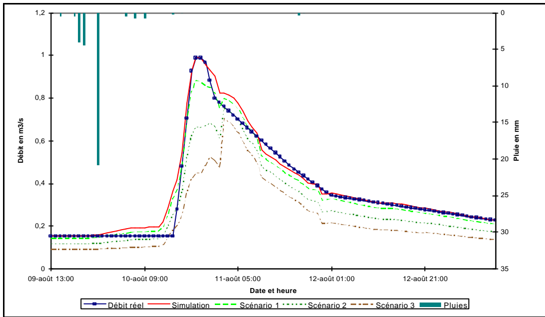
FIGURE 2 August 10, 1994 flood simulation for the actual situation and according to three scenarios of new upstream dams implementation. Scenarios 1, 2 and 3: 100, 300 and 500 dams in the downstream watershed preferential zone.
