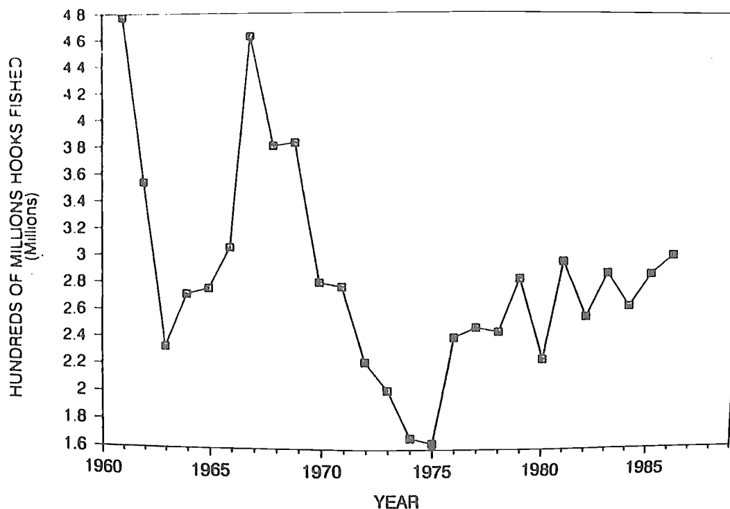
Figure 3. Estimated effective-effort for albacore by the Japanese longline fleet.
