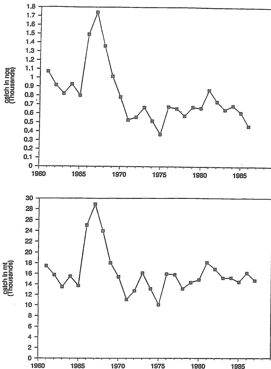
Figure 2. Japanese fleet longline catch in weight (upper panel) and numbers (lower panel).
