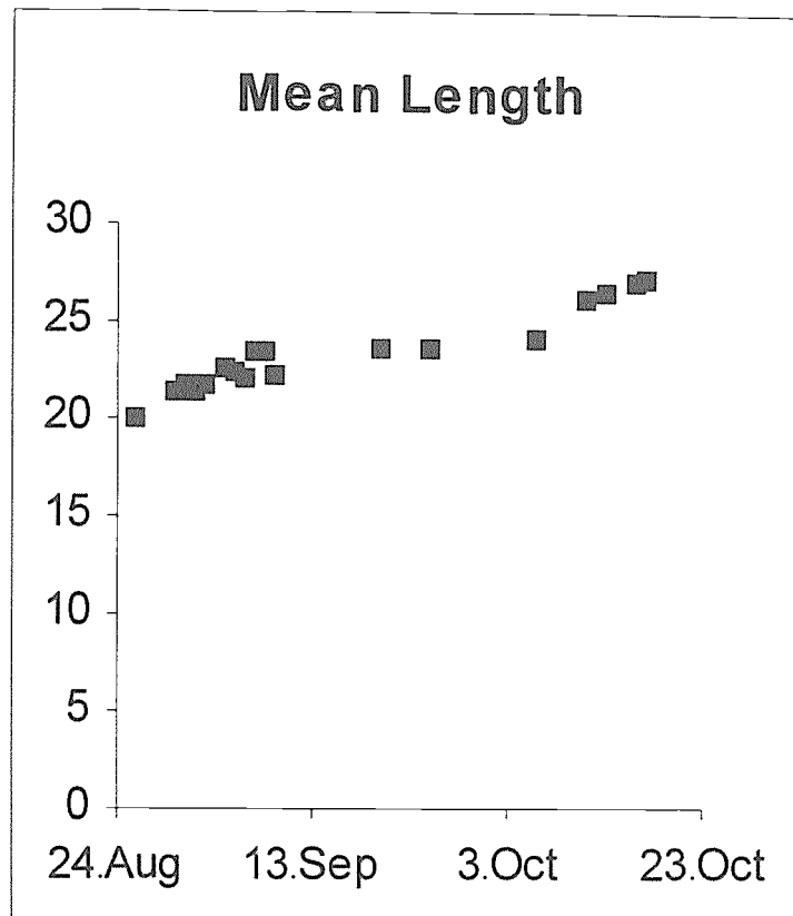
Figure 1. Mean lengths of juvenile kawakawa captured off Aburatsu, Japan during August-October (data from Yabe, 1953).
