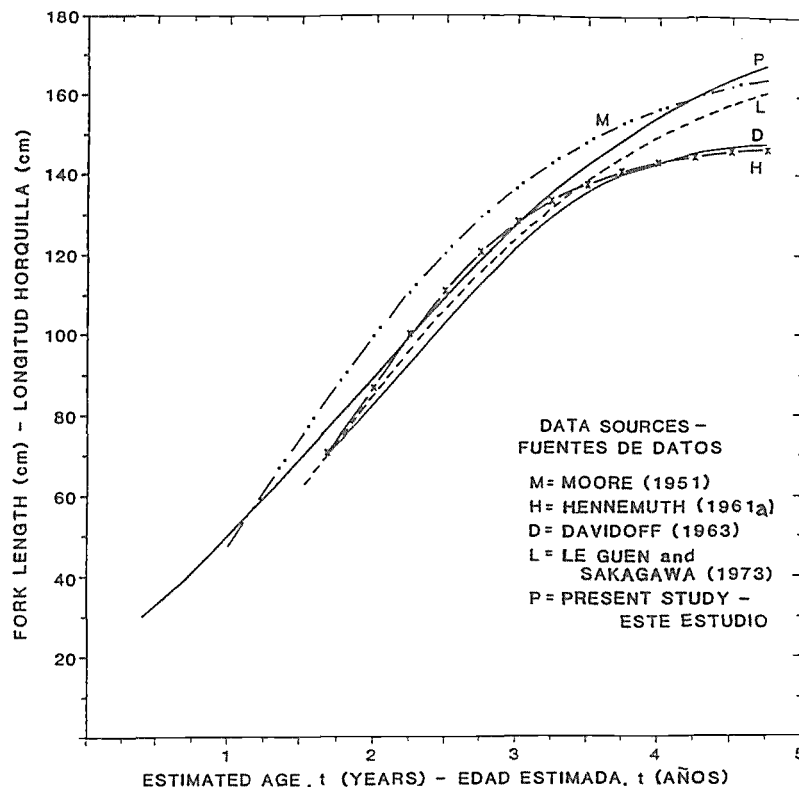
Figure 2. The fork-length growth curve (P) of yellowfin tuna in the eastern Pacific based on otolith-increment age estimates compared to previous curves derived from size-frequency analysis. (Reproduced from Wild, 1986.)
