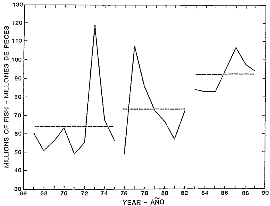
Figure 16. Estimated initial recruitments of yellowfin in the eastern Pacific Ocean, with the average recruitments for 1967-75, 1976-82, and 1983-89. (Reproduced from IATTC, 1991a).
