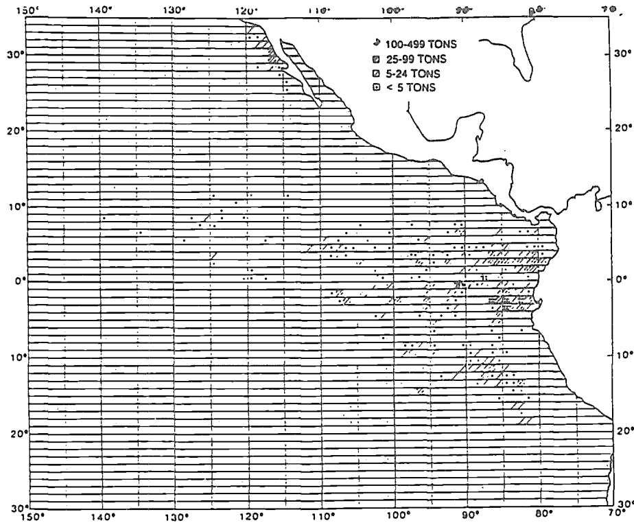
Figure 10. Annual average of distribution of bigeye catch by the eastern Pacific surface fishery, 1982-1986. (After Calkins et al. , 1988).
