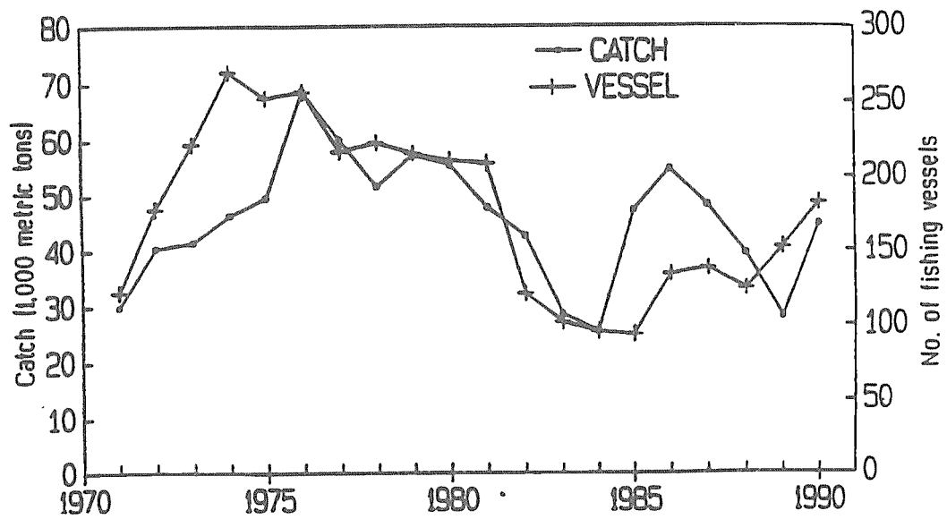
Figure 1. Trend in total catch and fishing vessels for Korean tuna longline fishery in the Pacific Ocean, 1971-1990.
