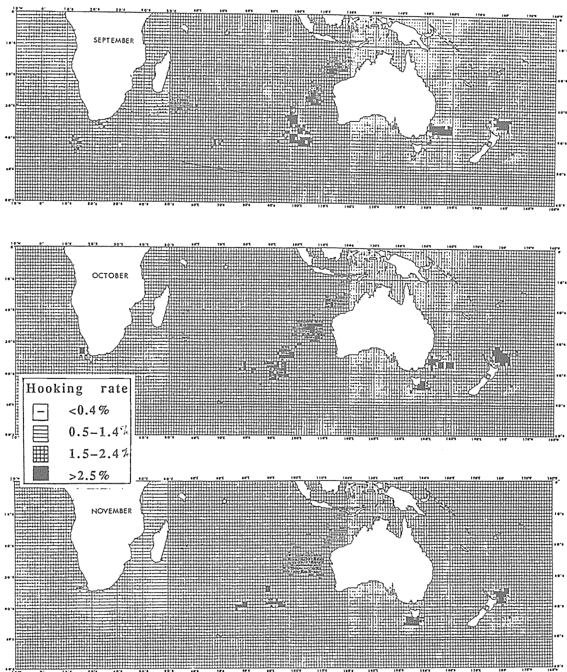
Figure 8. September to November changes in extent of longline fishing grounds and in average hooking rate for 1965-67. (Source: Shingu, 1970.)
