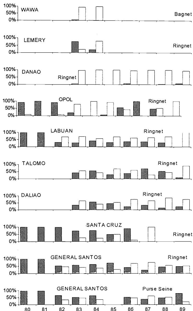
Fig. 6. Percentage species composition of Auxis catches by various fishing gears at nine landing sites in the Philippines (filled bar-frigate tuna; clear bar-bullet tuna).
