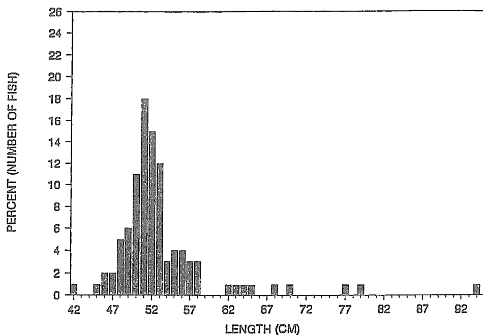
Figure 5. Length composition of yellowfin tuna caught by the Hawaiian artisanal handline fishery, 1978.
