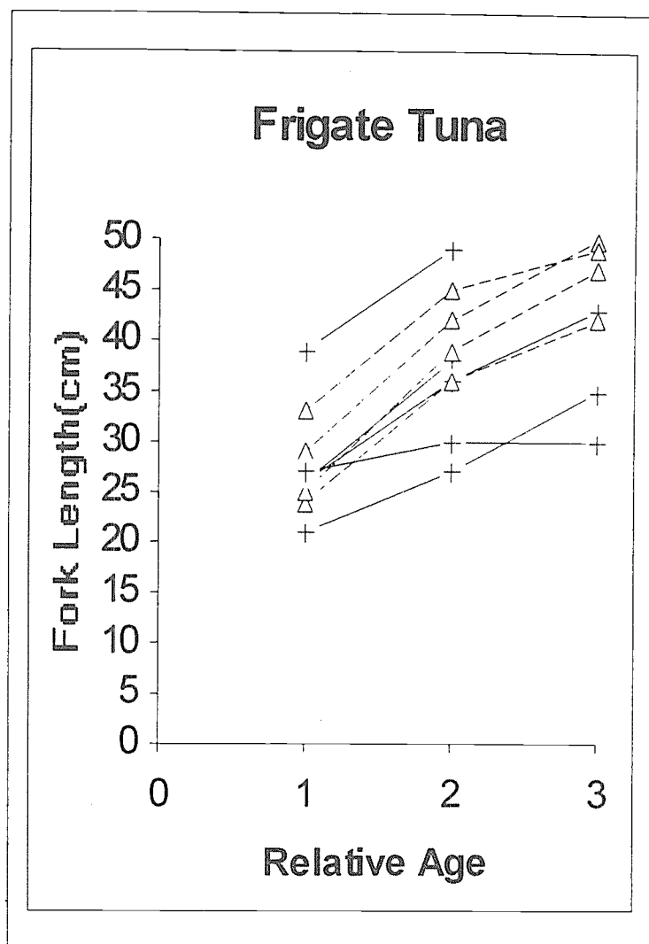
Fig. 19. Estimates of growth and relative age(years) of frigate tuna from length- frequency analyses (crosses-manual method; triangles-computer programmes).
