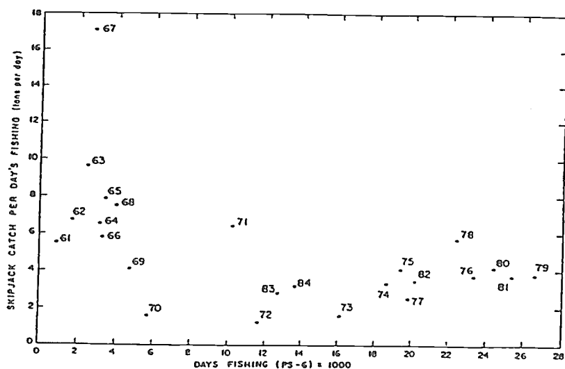
Figure 13. Plot of catch per days fishing (CPDF) and effort for skipjack in the EPO using data for all 5° areas. (After IATTC, 1985).
