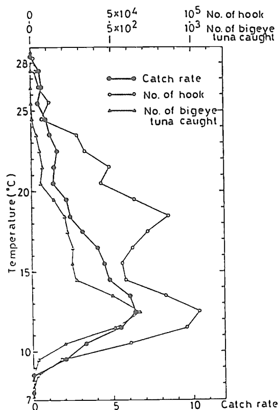
Figure 4. The catch, catch rate of bigeye tuna and the number of hooks used by water temperature at the depth of capture. (After Hanamoto, 1987).
