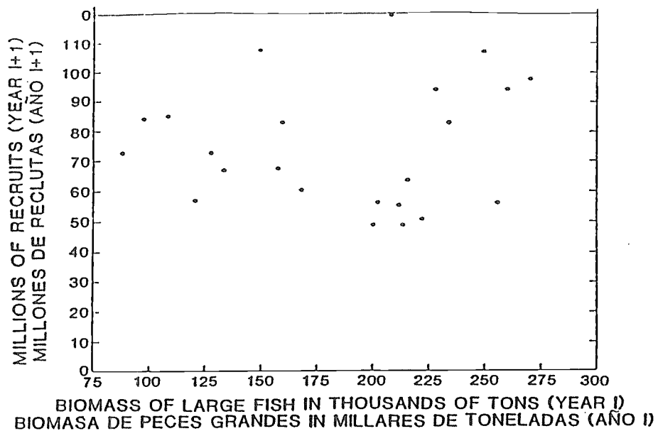
Figure 17. Relationship between stock and recruitment for yellowfin in the eastern Pacific Ocean for 1967 through 1989. Each dot represents the average recruitment of the X and Y cohorts. (Reproduced from IATTC, 1991a).
