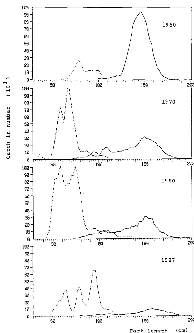
Figure 10. Length-frequency distribution of southern bluefin tuna caught by Australian surface fishery (dotted line) and Japanese longline fishery (solid line) in 1960, 1970, 1980, and 1987.
