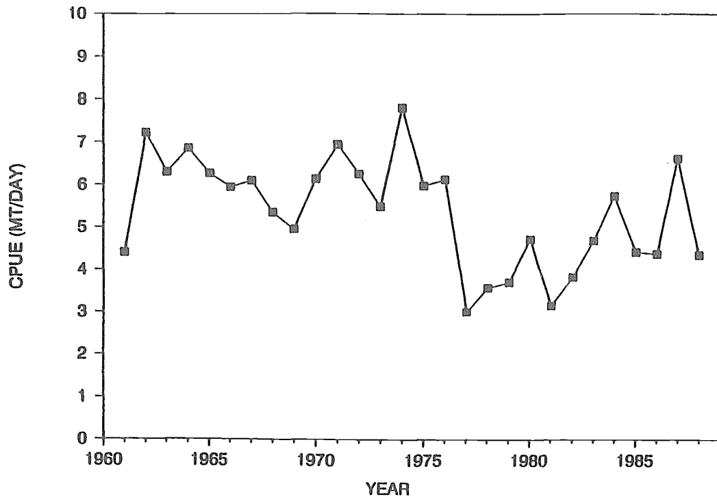
Figure 7. Estimated catch-per-unit-effort for albacore in the Japanese pole-and-line fleet.
