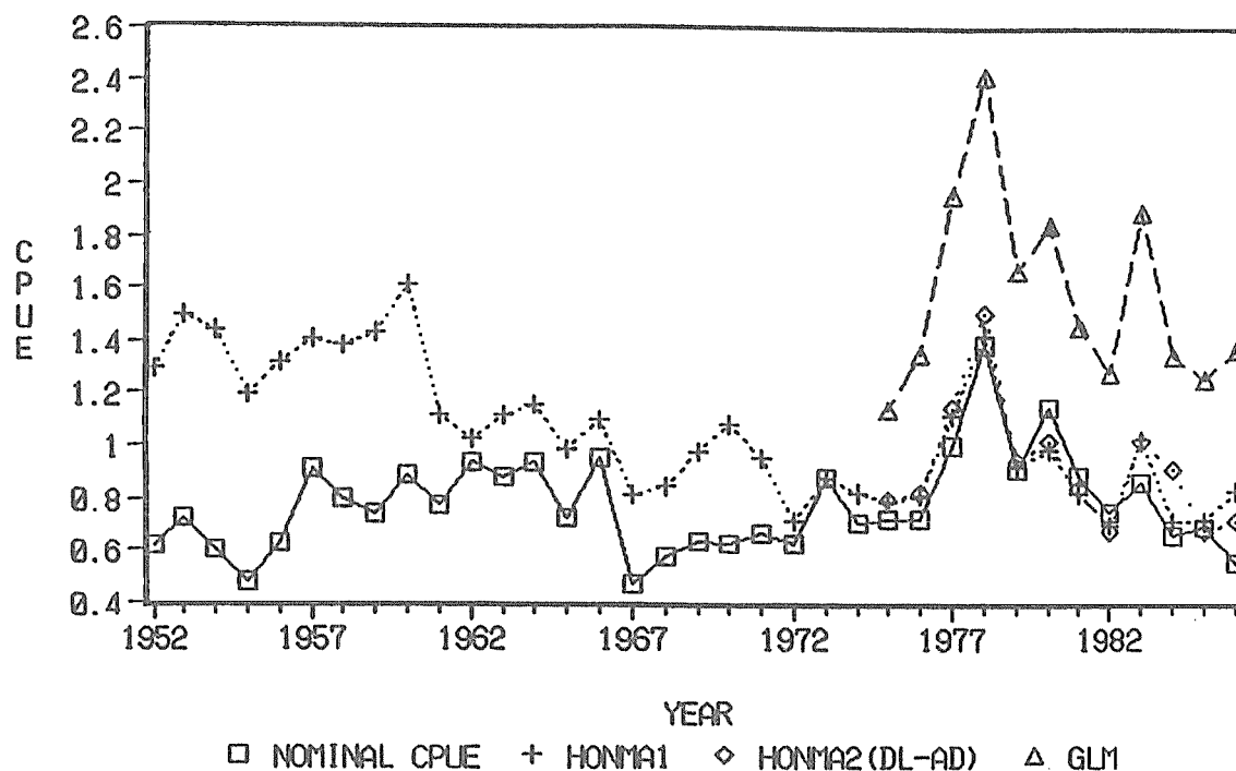
Figure 3. Trend of CPUE for yellowfin taken by the Japanese longline fishery in the western Pacific. (After Suzuki et al. , 1989). The HONMA1, HONMA2(DL-AD), and GLM denote Honma's method without deep and regular longline adjustment, with adjustment, and general linear model, respectively.
