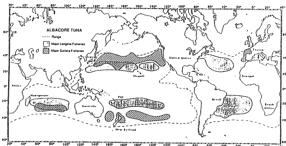
Figure 1. General distribution of albacore showing distribution of major surface and longline fisheries.
