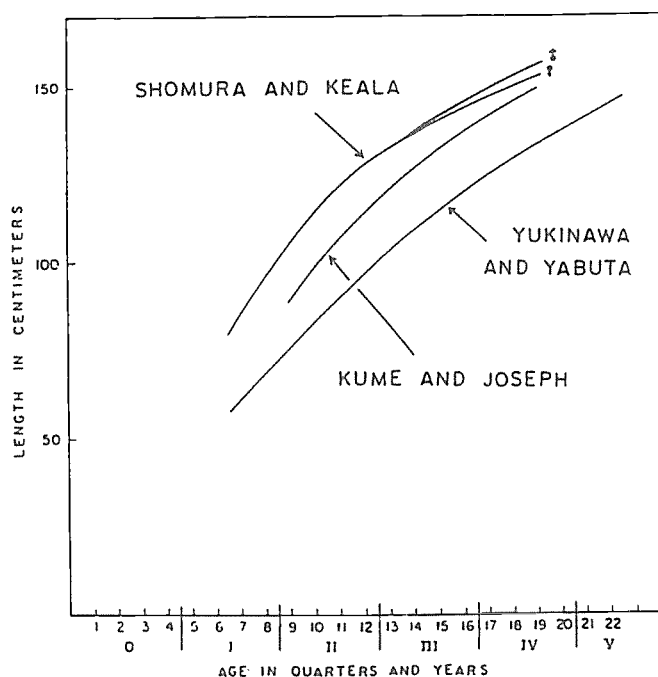
Figure 2. Growth curves of bigeye tuna estimated by various authors. (After Kume and Joseph, 1966).
