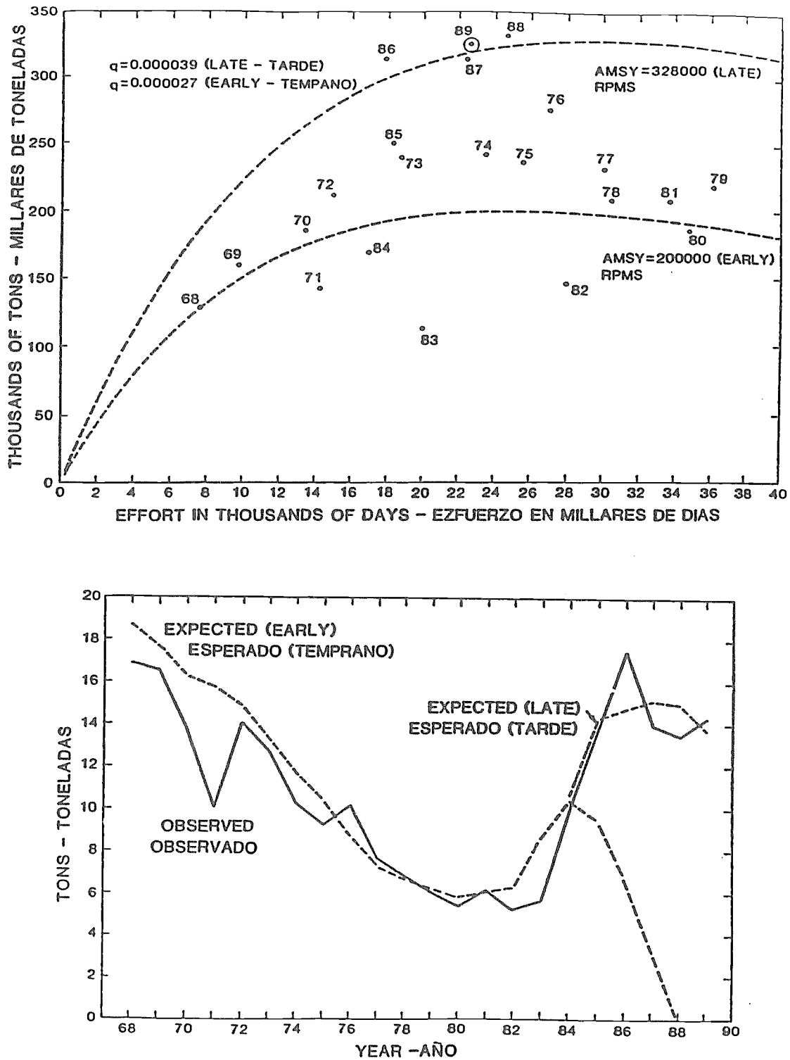
Figure 20. Relationships between effort and catch for the yellowfin fishery in the eastern Pacific Ocean during 1968-89 for the generalized stock production (asymmetrical) model with m set at 0.8 (upper panel), and observed and predicted values of CPDF (lower panel). (Reproduced from IATTC, 1991a).
