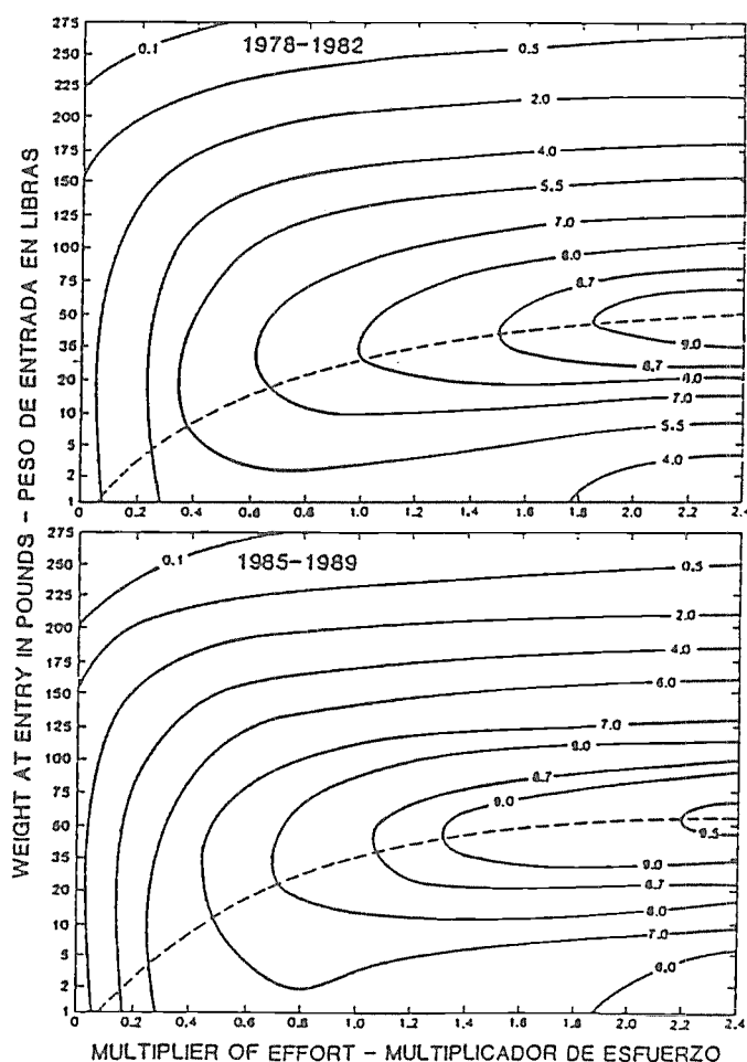
Figure 18. Relationships among size at entry, fishing effort, and yield per recruit for yellowfin for two different patterns of age-specific fishing mortality. (Reproduced from IATTC, 1991a).
