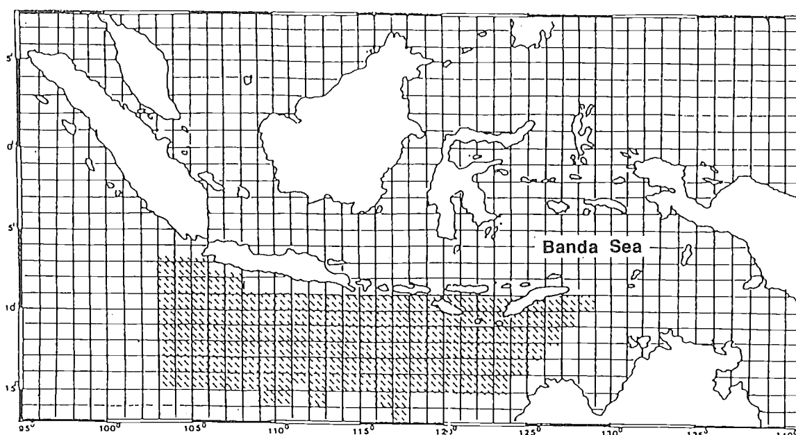
Figure 9. Yearly fishing grounds of southern bluefin tuna in southern Java and Nusatenggara waters, 1978-88. (Source: Bahar and Naamin, 1989.)
