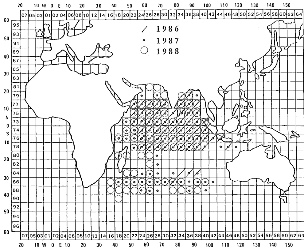
Figure 10. Distribution of annual Taiwanese "deep" longlining effort in the Indian Ocean, 1986-88. (Source: Hsu and Liu, 1990.)
