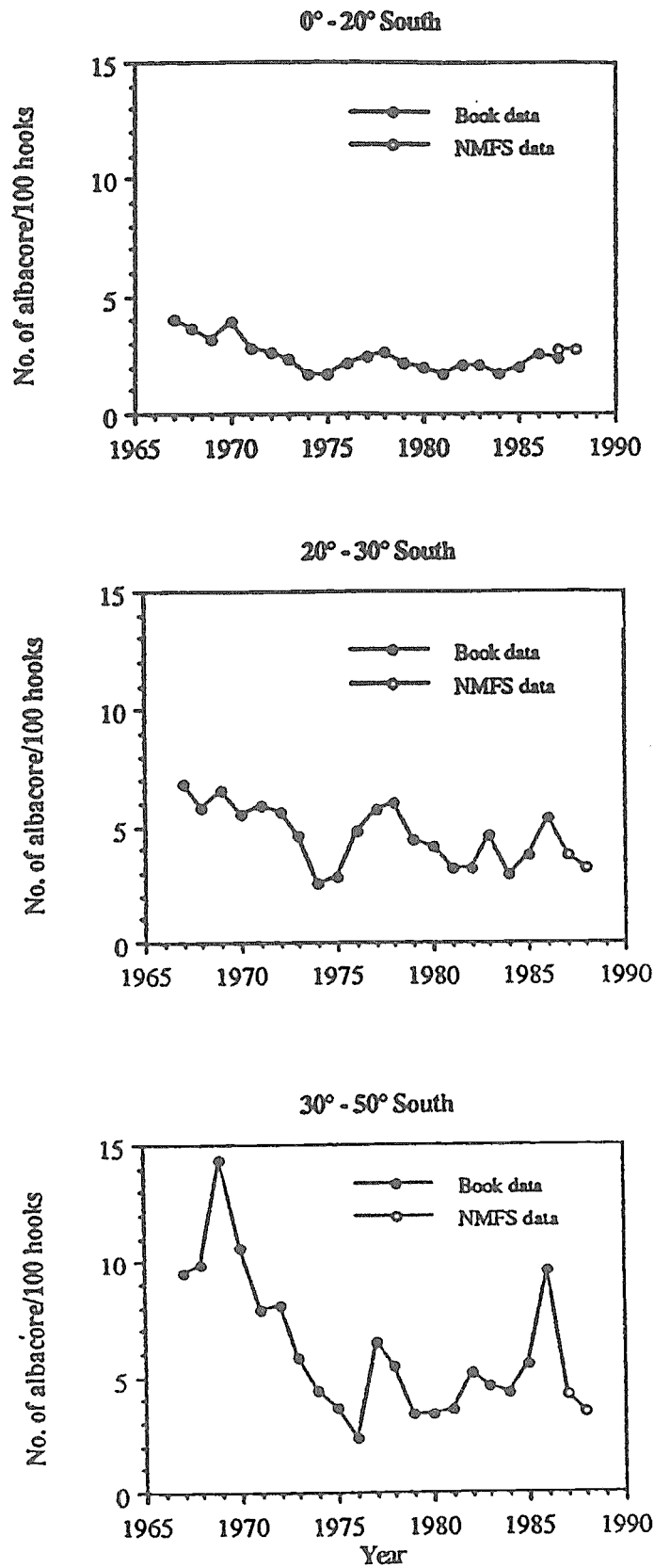
Figure 2. CPUE trends in South Pacific albacore longline fisheries stratified by latitude. Reprinted from Anon (1991).
