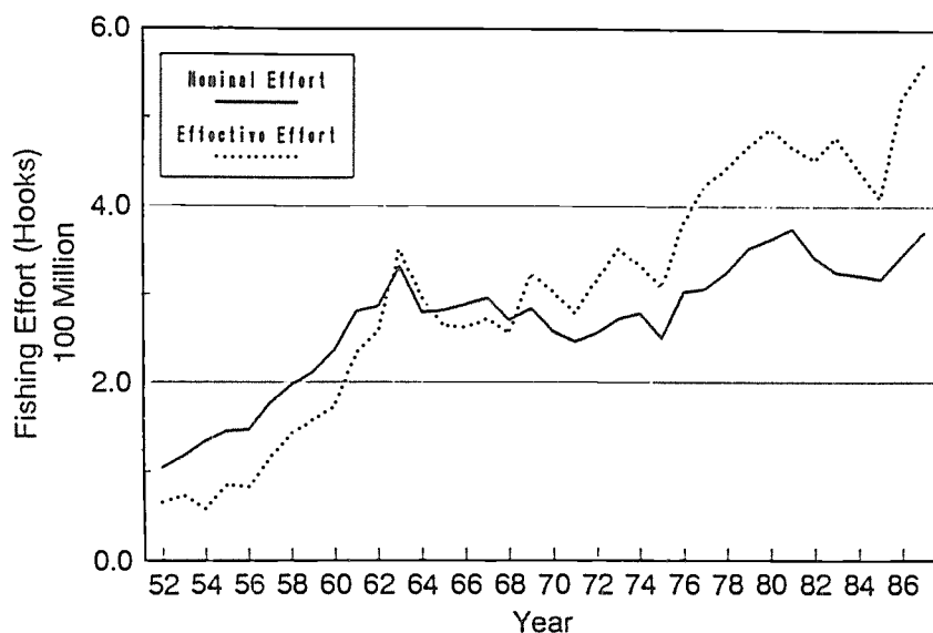
Figure 12. Annual trend of fishing effort by Japanese longline fishery. (After Miyabe, 1991).
