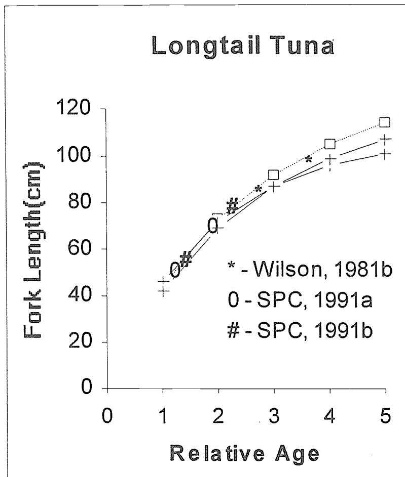
Figure 2. Growth curves derived from otolith increment counts (squares) and length-frequency distributions (crosses) with growth increments of long-term tag recoveries of longtail tuna.
