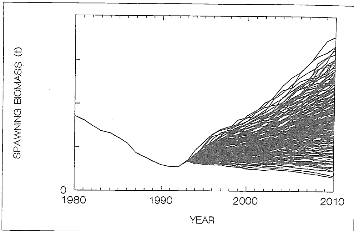
Figure 22. Indicative trajectories of future southern bluefin tuna spawning stock tonnage to year 2010 under the current quota regime (121,500 mt globally) and assuming continuation of the historic range of variability in recruit production relative to spawning stock tonnage. Absolute spawning stock tonnages are not shown because they vary with VPA estimates generated and with the stock-recruitment relationship assumed.
