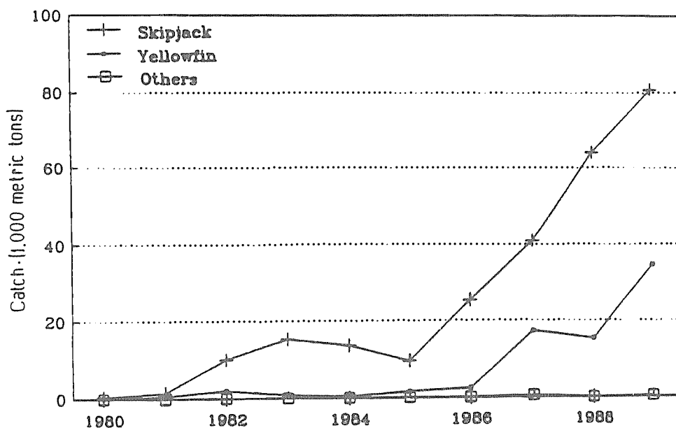
Figure 4. Trend in catch of tunas by Korean tuna purse-seine fishery in the western Pacific Ocean, 1980-1989.
