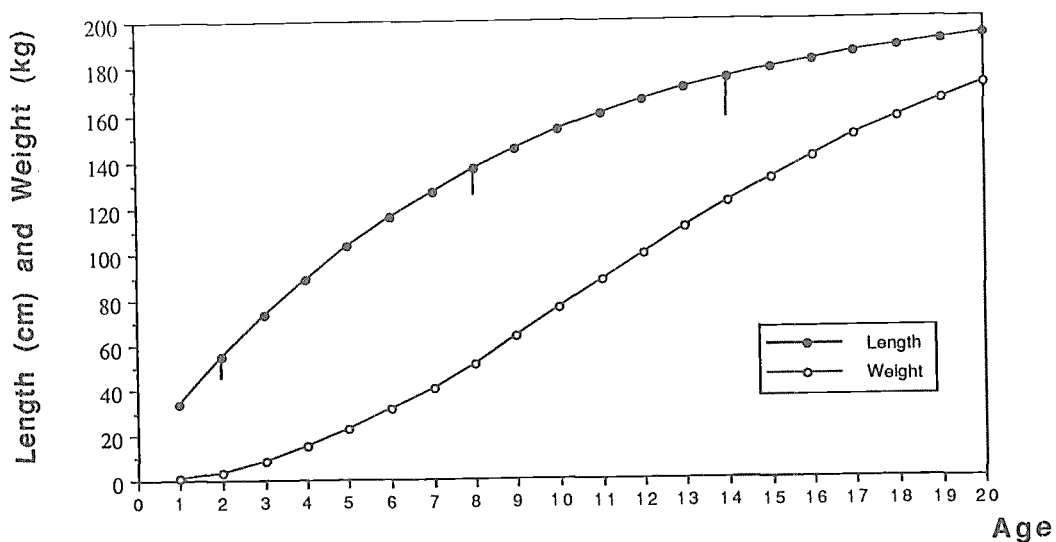
Figure 4. Growth in length* and weight of southern bluefin tuna. Values of von Bertalanffy growth parameters for the length curve area K=0.128 per year; t=-0.394 years; and L=207.6 cm. Growth in weight is derived from the length-weight relationships in Figure 5. (* The bars on the length curve represent the range of length at ages 2, 8, and 14 years for the different von Bertalanffy parameters derived for southern bluefin tuna.)
