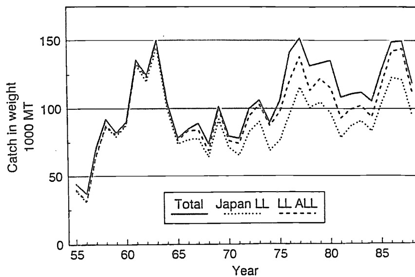
Figure 13. Annual catch trend of Pacific bigeye tuna.
