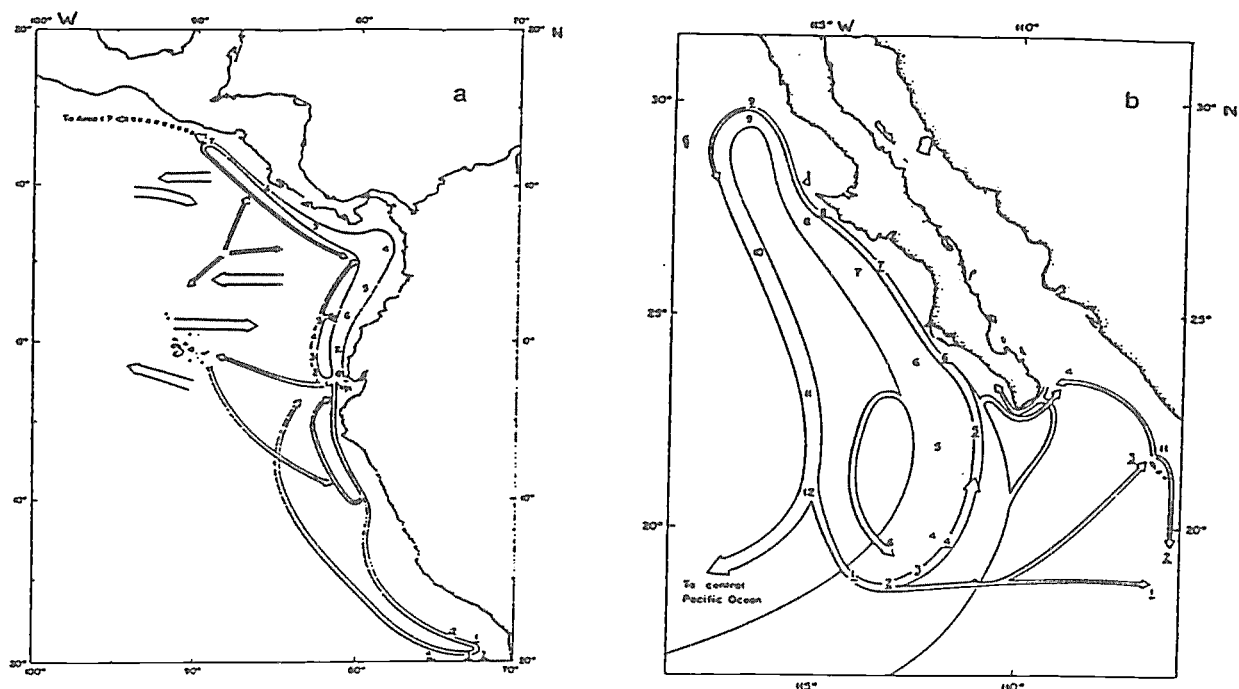
Figure 8. Migratory paths of skipjack entering (a) to the south and (b) to the north in the eastern Pacific. (After Fink and Bayliff, 1970).
