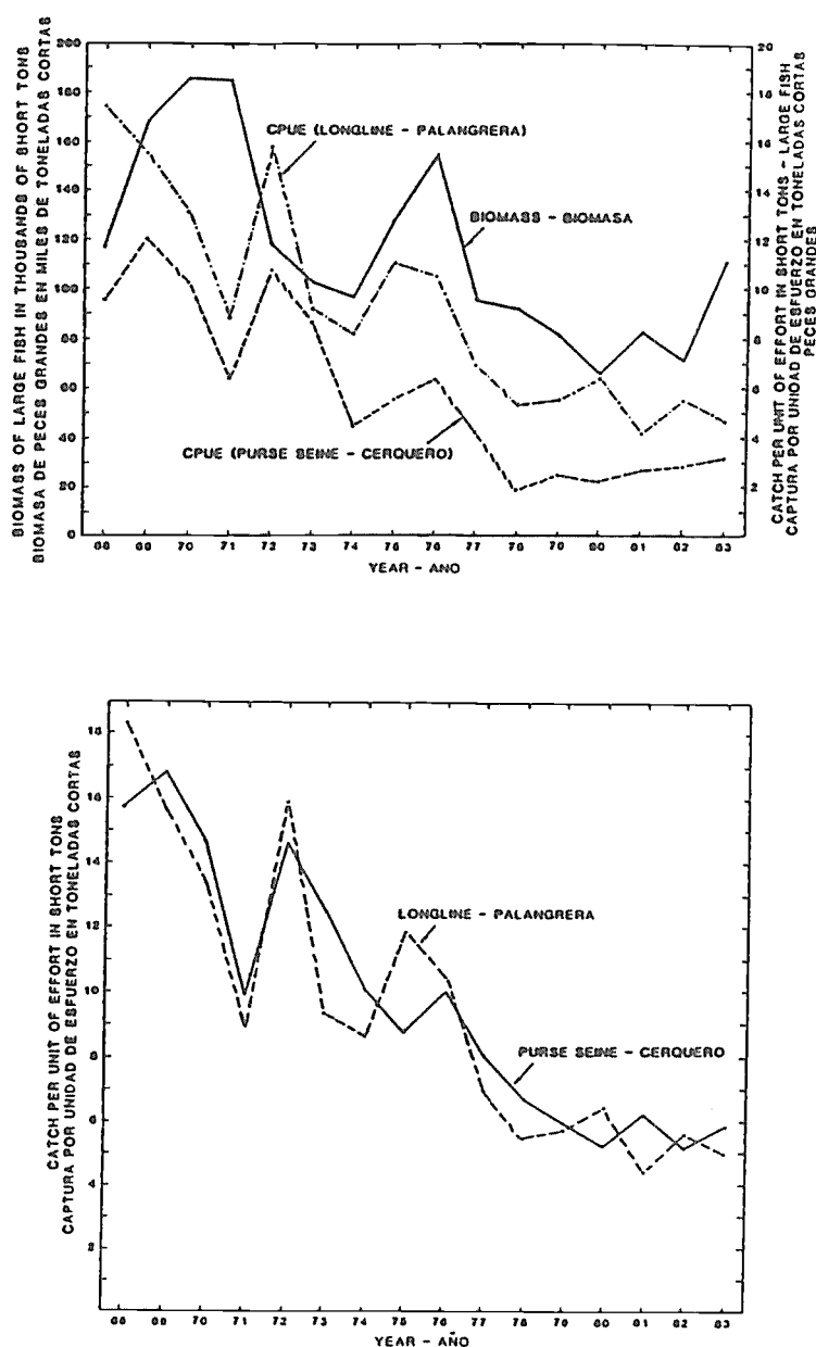
Figure 21. CPUEs of large yellowfin by Class-6 purse seiners and by longliners, compared to biomass estimates of large yellowfin (upper panel); and catch per day's fishing by Class-6 purse seiners, compared to catch of yellowfin per 73,800 hooks by longliners (lower panel). All comparisons are for the eastern Pacific Ocean east of 150°W. (Reproduced from IATTC, 1987).
