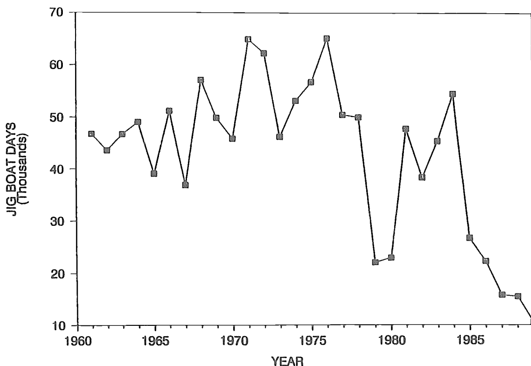
Figure 9. Estimated effort in the USA troll fishery.
