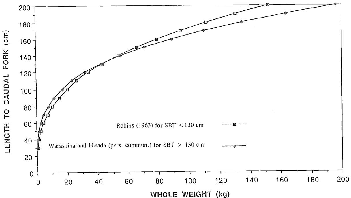
Figure 5. Relationships currently used to convert southern bluefin tuna weight to length; the relationship for southern bluefin tuna > 130 cm has been adjusted from a processed-weight; length relationship to a whole-weight:length relationship using a 1:1.15 ratio of processed to whole weight.
