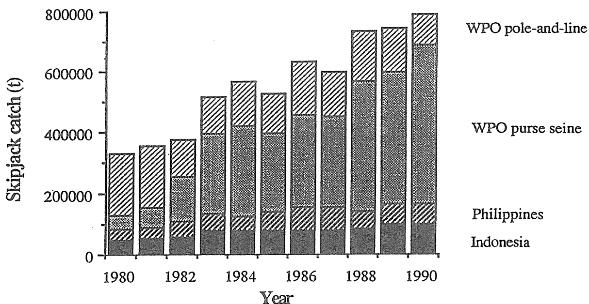
Figure 14. Catch trend for skipjack in the WPO. (After SPC, 1991).
