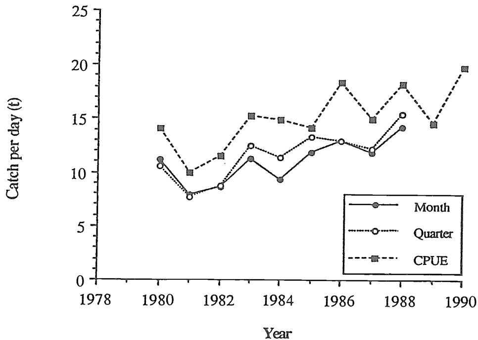
Figure 15. Various indices of skipjack apparent abundance based on CPDF in the Japanese purse-seine fishery. "CPUE" refers to unadjusted CPDF, "Month" refers to average CPDF stratified by month and 2° latitude by 5° longitude rectangular areas, and "Quarter" refers to average CPDF stratified by quarter and 2° latitude by 5° longitude rectangular areas. (After SPC, 1990).
