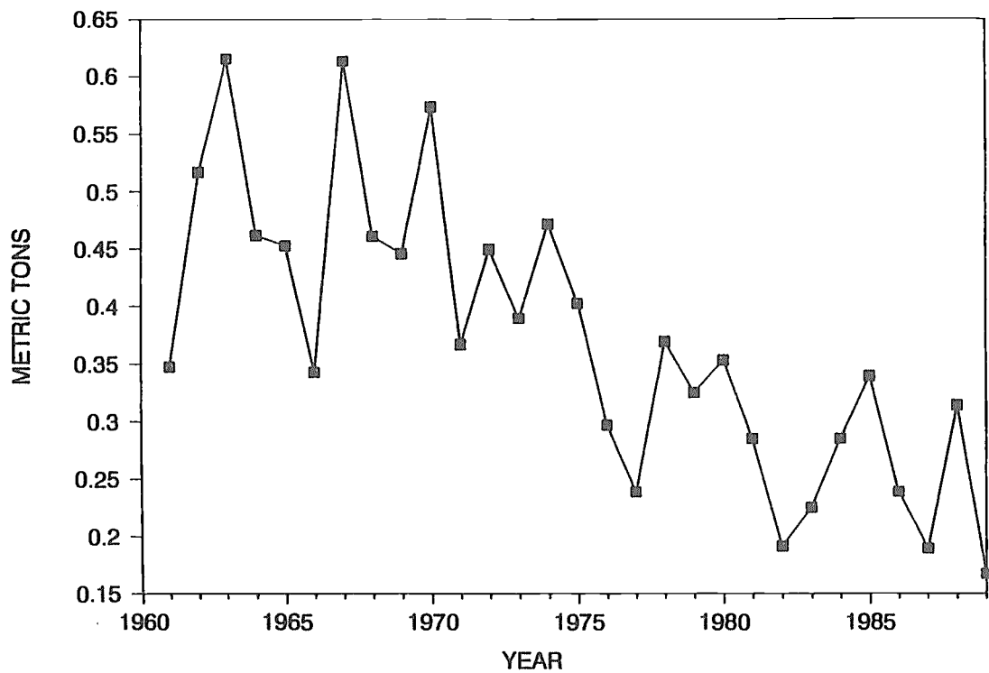
Figure 11. Estimated catch-per-unit-effort in metric tons per day per boat for the USA troll fleet.
