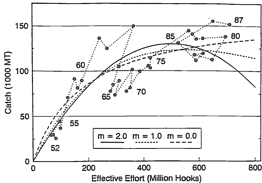
Fig. 17. Annual catch against annual fishing effort and estimated production curves for Pacific bigeye tuna. After Miyabe (1991).
