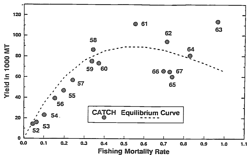
Fig. 18. The estimated equilibrium curve for Pacific bigeye tuna. After Suda and Kume 1967.
