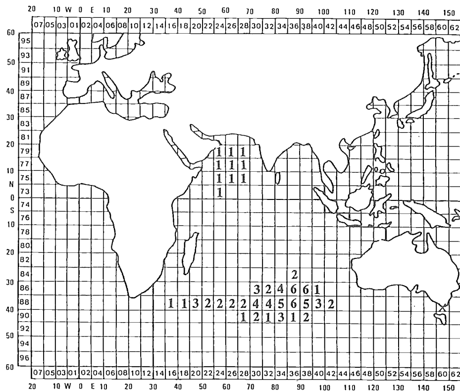
Figure 11. Accumulated number of months of Taiwanese large-scale pelagic drift gillnet effort in 5° squares in the Indian Ocean, 1987-88. (Source: Hsu and Liu, 1990.)
