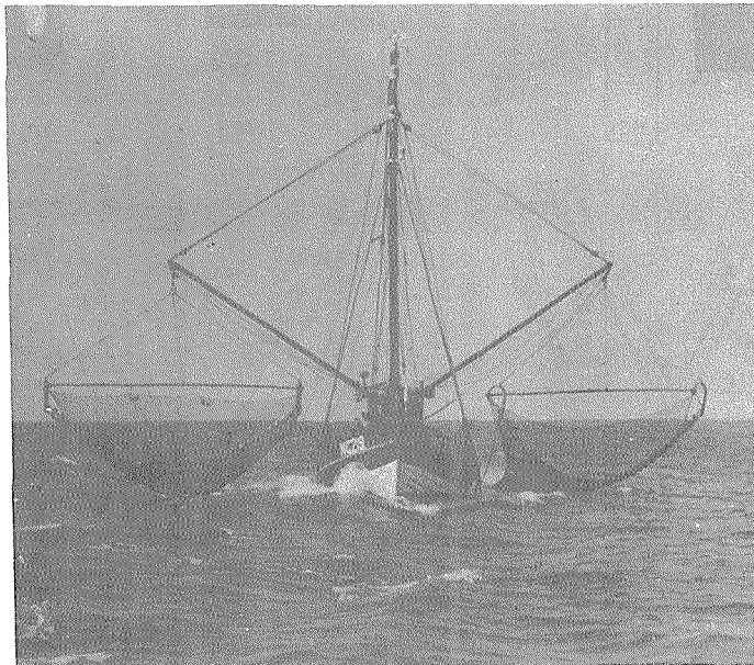
Fig. 17 Modern German shrimp fishing vessel from Cuxhaven (Meyer-Waarden and Tiews, 1957). (Photo: Dr. Nolte)
