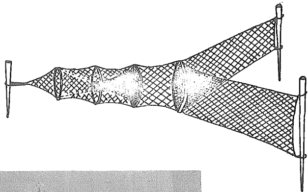
Fig. 16 German shrimp fyke net with wings (Meyer-Waarden, 1931).
