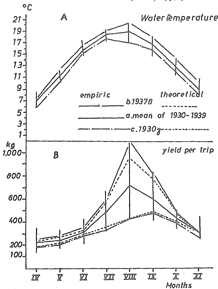
Fig. 13 Water temperature (A) and yield of shrimps per trip (B) given as monthly mean for a = 1930-1939, b = 1937 and c = 1930 in the Büsum area. The dotted curves ( \beta = 1937 and \gamma = 1930) are based on the water temperature - catch relationship found (Tiews, 1954b).
