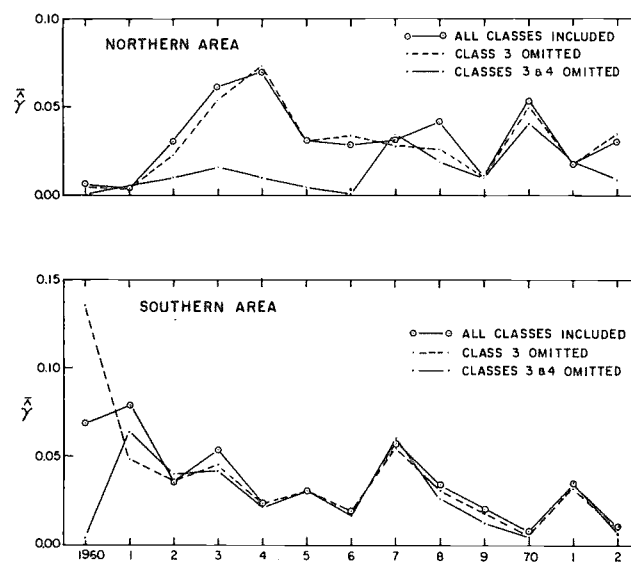
Figure 68.—Annual biomass indices of skipjack tuna in the traditional fishing areas of the eastern Pacific Ocean using different combinations of vessel classes, 1960-72 (from Pella and Psaropulos 1975).
