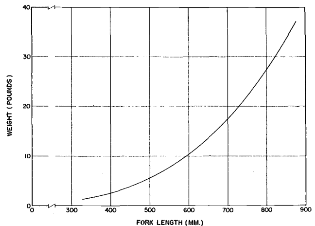
Figure 65.—Length-weight relation of skipjack tuna: \log \text{ weight} = -8.34241 + 3.36836 \log \text{ length} (parameters not corrected for transformation bias); number of observations, 1,298; size range, 327-877 mm; data collection period February 1948-December 1960; from files of Southwest Fisheries Center (from Nakamura and Uchiyama 1966).
