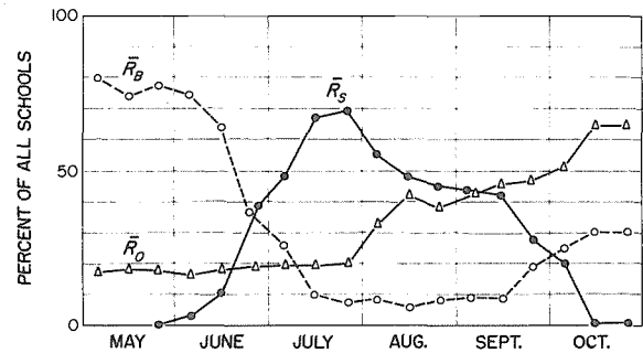
Figure 45. —Ratio of detection of schools with birds ( \bar{R}_B ), schools without birds ( \bar{R}_O ), and schools with sharks ( \bar{R}_S ) to total schools in each 10-d period (from Kimura 1954).
