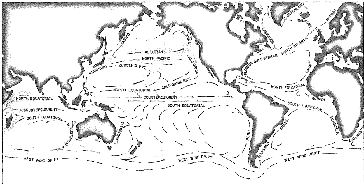
Figure 15.—Ocean current systems (from Brock 1959).
