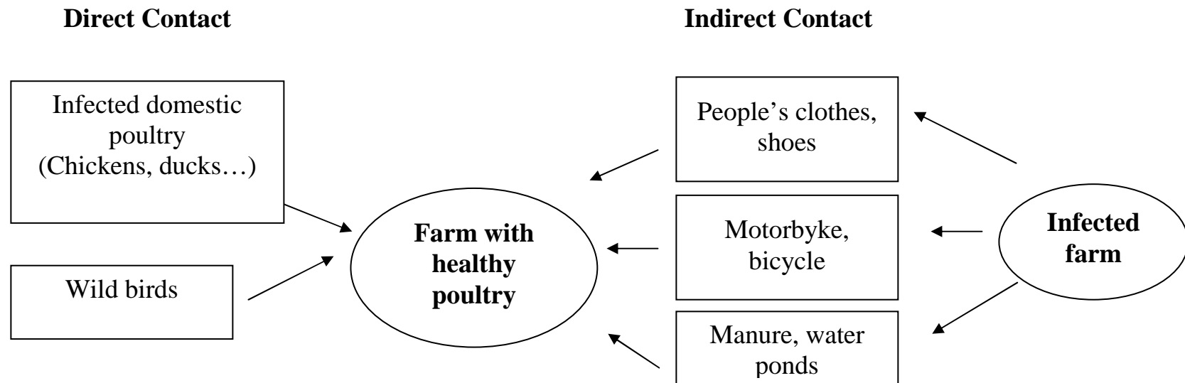
Figure 1: Possible direct and indirect contacts between infected and non-infected poultry that can bring Avian Flu in a farm.
