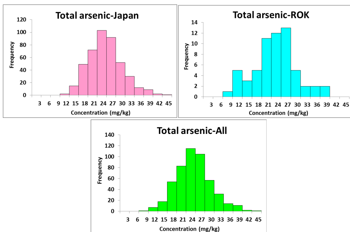
Fig 1: Histogram of total arsenic concentrations in laver products
