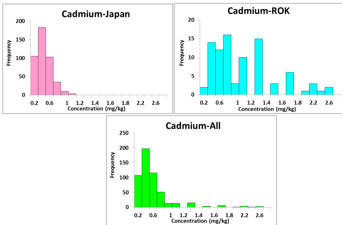
Fig 2: Histogram of cadmium concentrations in laver products
