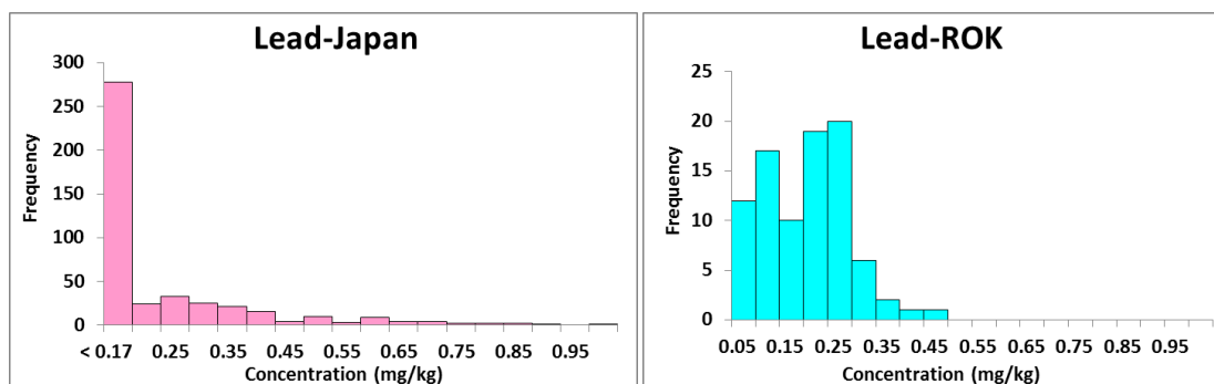
Fig 3: Histogram of lead concentrations in laver products (*)
