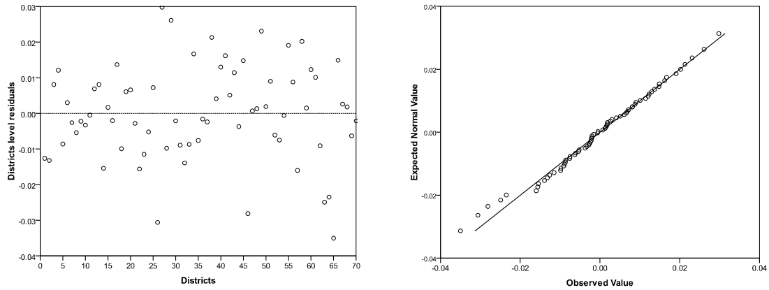
Figure 1. Distribution of the district level residuals (left hand side) and normal q-q plot of the district level residuals (right hand side)
