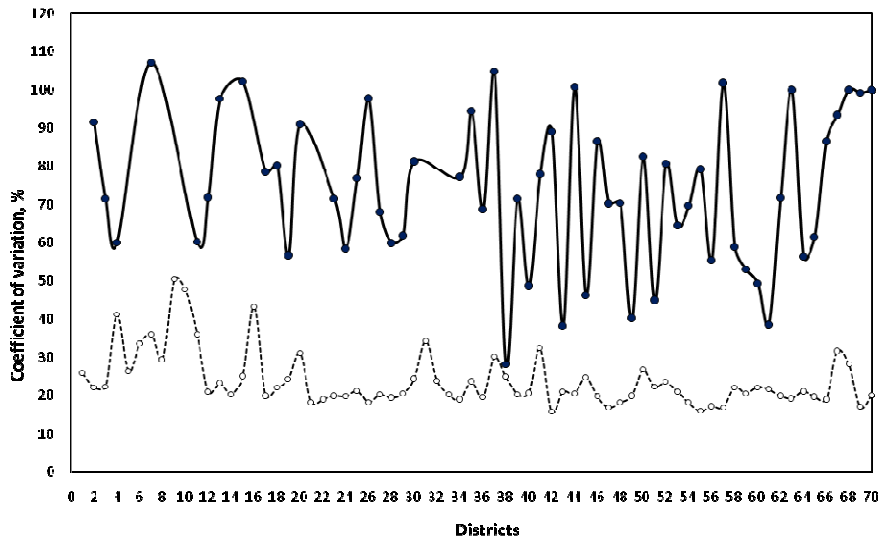
Figure 3. District-wise coefficient of variation for direct (solid line) and model-based estimate (dash line)
