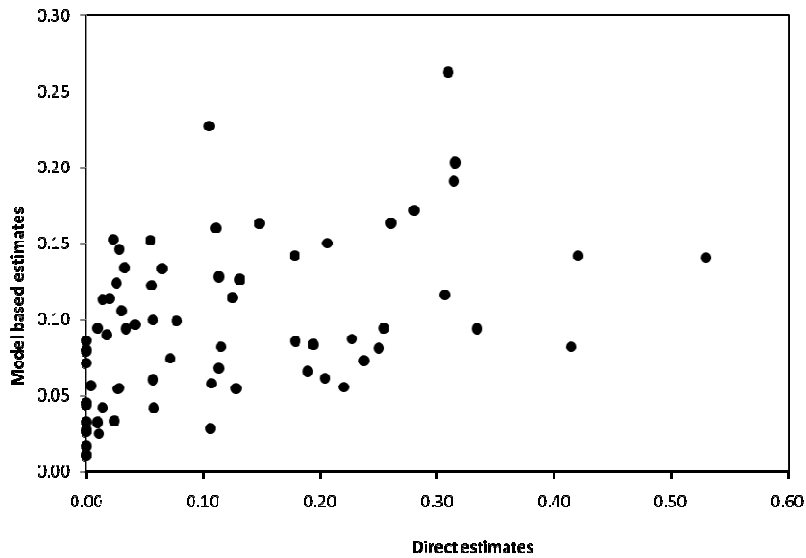
Figure 2. Bias diagnostics plot
