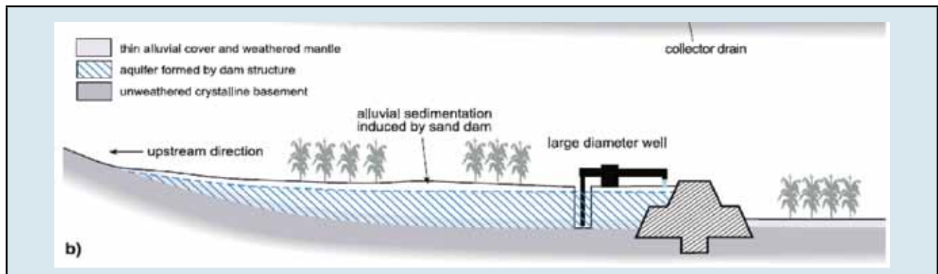
Figure 3.6: Cross section of Sand Dam Structure (from Foster and Tuinhof, 2004)
