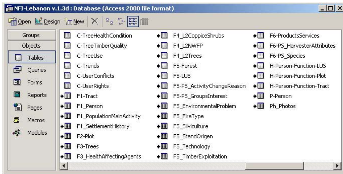
Figure 6: Database window in the NFA application database (" NFI- \langle COUNTRY \rangle v.x.x.mdb ") showing some of the code tables in the database (beginning with "C-") and some of the linked data tables (with an arrow symbol next to the table symbol).
