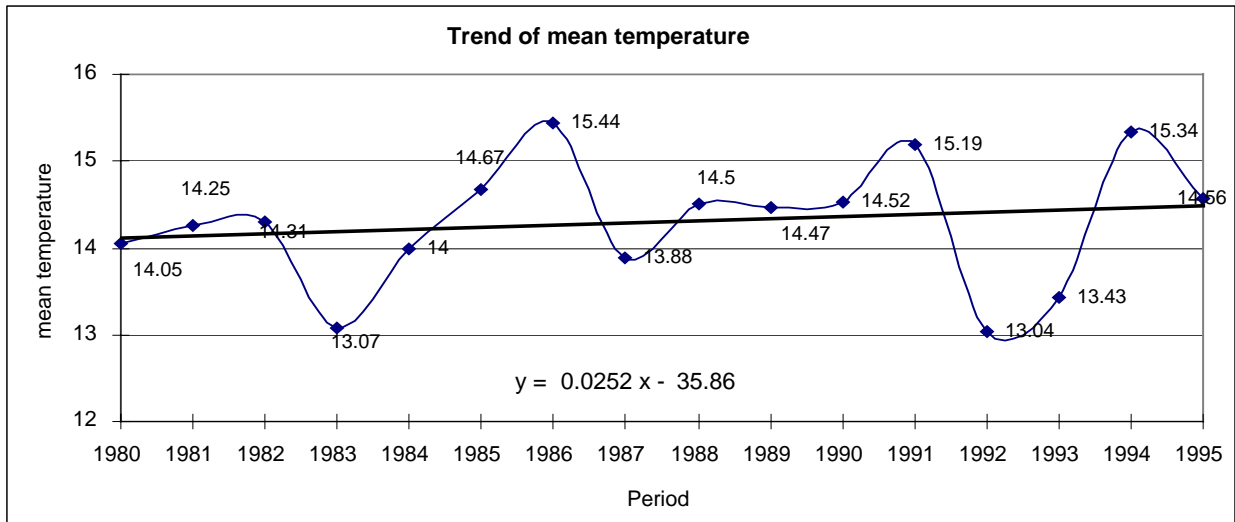
Fig.(1) Trend of temperatures at Elmansoura location from the 1st period of January to the 2nd period of April during the period 1980-1995
