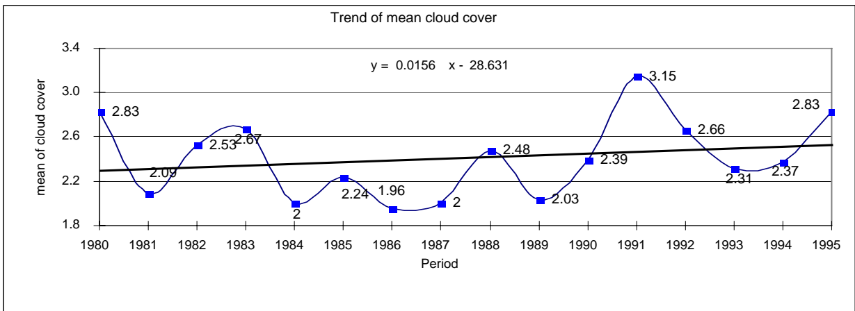
Fig.(3)Trend of cloud, wind and misty days at Elmansoura location from the 1 st period of January to the 2nd period of April during the period 1980-1995
