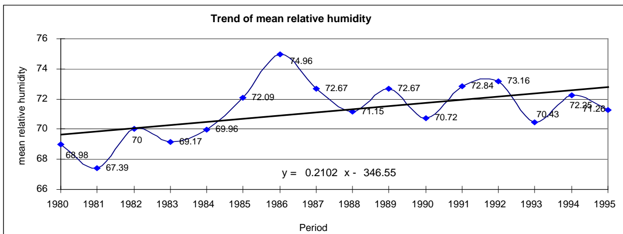
Fig.(2) Trend of relative humidities at Elmansoura location from the 1st period of January to the 2nd period of April during the period 1980-1995
