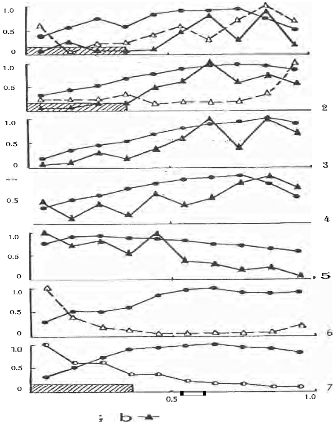
Figure 31.— The horizontal drift distribution of young fish under velocity gradient conditions: Diags. 1-5, during the hours of darkness; Diag 6, during daylight hours and, Diag 7, the comparable drift of dead fish . a. = velocity curve across width of chute, b. = distribution of fish in natural drift, \square = distribution of fish released at 1st section, \square = distribution of dead fish. X axis = chute length in \square , Y axis = relative concentration of fish (N) and relative flow velocity (V) cross hatching = part of chute where fish are released.
