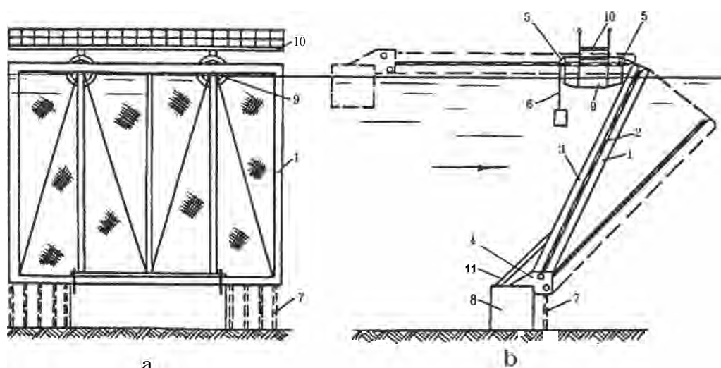
Figure 22.— A mechanical guiding device: a. front elevation, b. section: after Malevanchik & Nikonorov (1984). 1. frame, 2. fish-protection screen (FPL), 3. tube of pontoon, 4. hinge connection, 5. block system, 6. counterbalance of FPL, 7. chains, 8. bottom pontoon, 9. support pontoon, 10. access bridge, 11. hose for filling pontoon with water or air.
