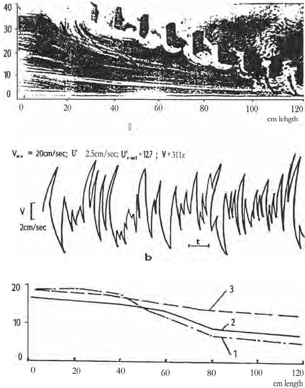
Figure 37.— a. Flow structure in front of a barrier composed of L-shaped plates at 8cm intervals, b. Pulses of current velocity 5cm in front of barrier in cross section: V_{av} = 20\text{cm/sec} ; t = 1 sec; U' = 2.5\text{cm/sec} ; U'_{rel} = 12.7\% ; c = 3.1 hertz, c. Lines of fish movement: 1. in light, 2. in darkness, 3. of dead fish.
