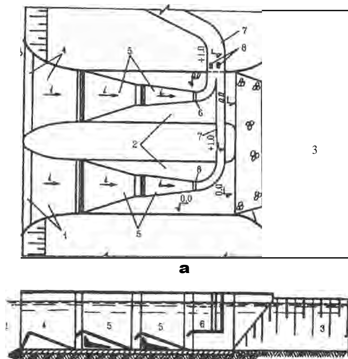
Figure 35.— Diversion device based upon differences in the vertical distributions of fish; a. in plan, b. in cross section (after Malevanchik & Nikonorov, 1984): 1. water intake basin, 2. water supply canal, 3. water intake canal, 4. entrance section, 5. concentrating
