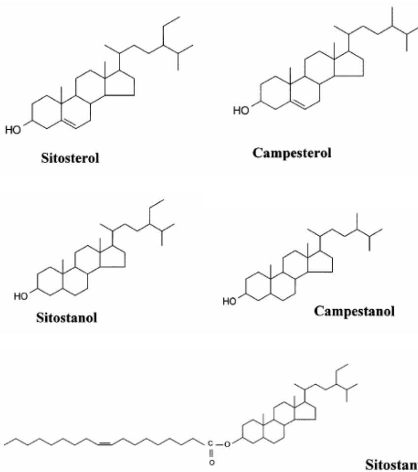
Figure 2. Molecular structure of some phytosterols, phytostanols and a fatty acid ester.
