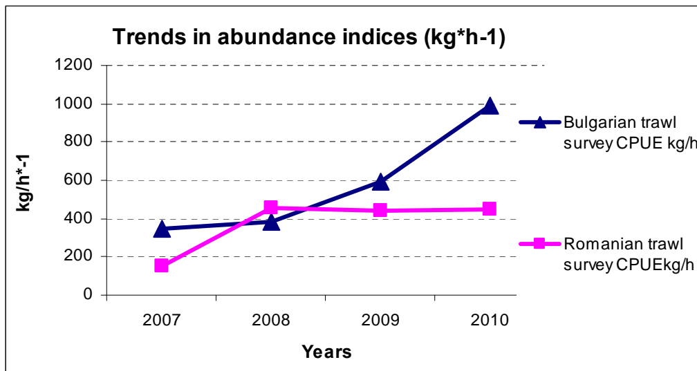
Figure 4.4: Trends in abundance (CPUE kg.h^{-1} ) derived from Bulgarian and Romanian pelagic trawl surveys.
