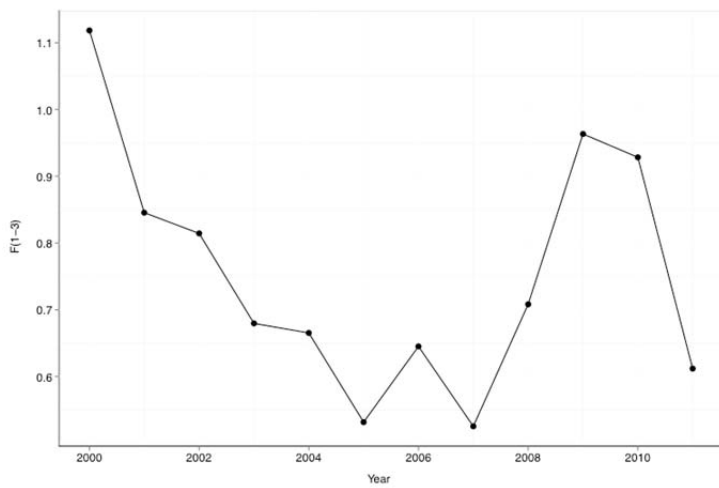
Figure 8.3: F_{\bar{bar}(1-3)} estimates.
