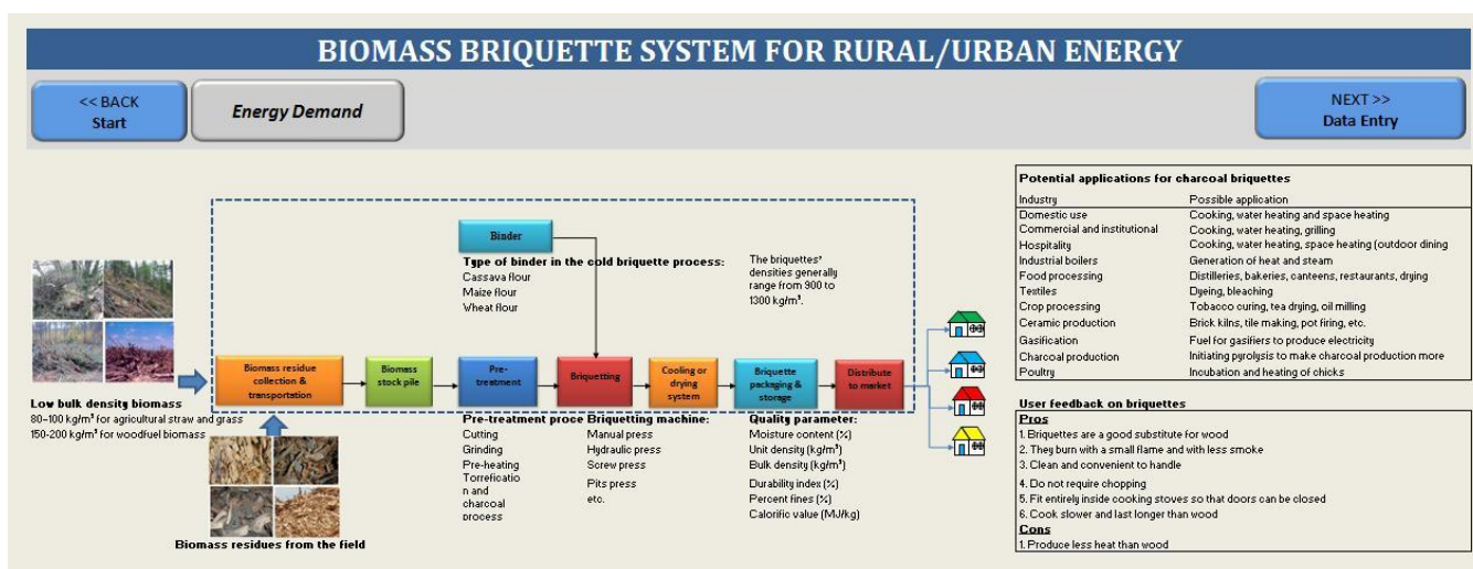
Figure 2: Biomass Briquette System for Rural and Urban Heating and Cooking
