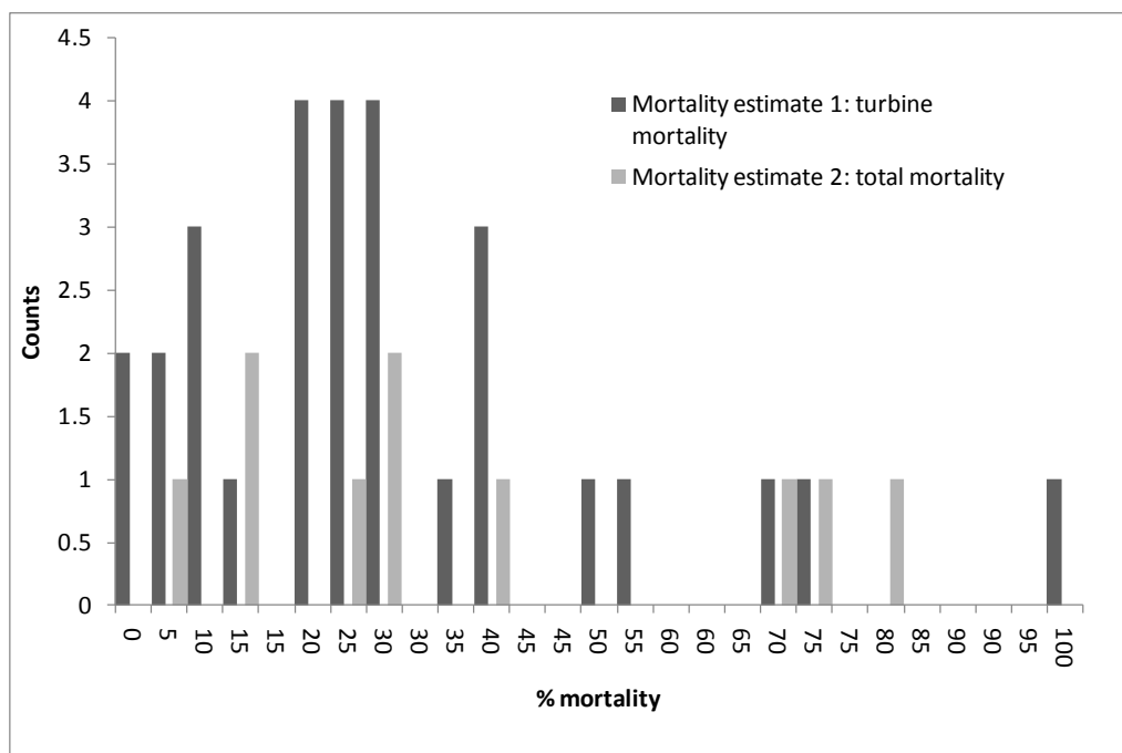
Figure 4-4. Distribution of mortality estimates based on Table 4.1.
