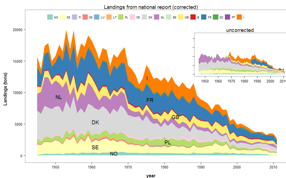
Figure 2-10. Total landings (all life stages) from 2011 Country Reports (not all countries reported); the corrected trend has missing data filled by GLM.
