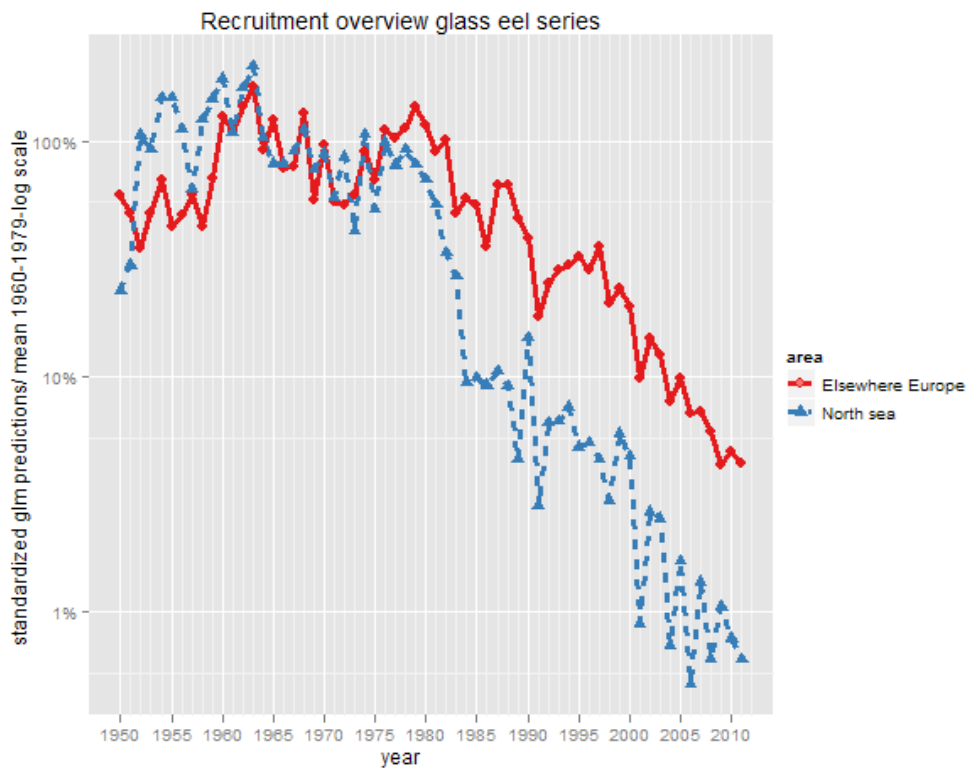
Figure 2-5. WGEEL recruitment index: mean of estimated (GLM) glass eel recruitment for the continental North Sea and elsewhere in Europe. The GLM ( \text{recruit}=\text{area}:\text{year}+\text{site} ) was fitted to all glass eel series available and scaled to the 1960–1979 average. No series for glass eel are available in the Baltic area. Note logarithmic scale on the y-axis .
