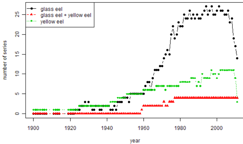
Figure 2-2. Trend in number of available dataserries per life stage.
