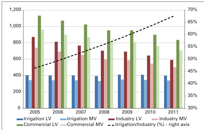
FIGURE 31 Cost of electricity for irrigation and to industry and commerce (in Kip/kwh constant 2011 prices)
