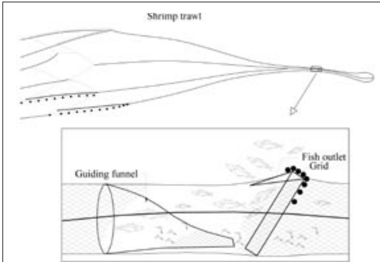
Shrimp trawl with sorting grid (expanded view). Shrimp and fish that pass backwards in the trawl are guided by a funnel to the bottom of the backwards slanting metal grid. Shrimp and fish of comparable size will pass through the slots of the grid and go to the codend, while larger fish and other organisms (e.g. jellyfish) will slide upwards over the grid and are released through the outlet.
