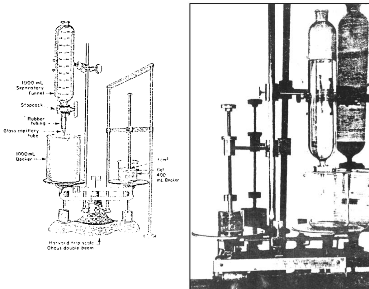
Fig. 15. Rowerbal method
