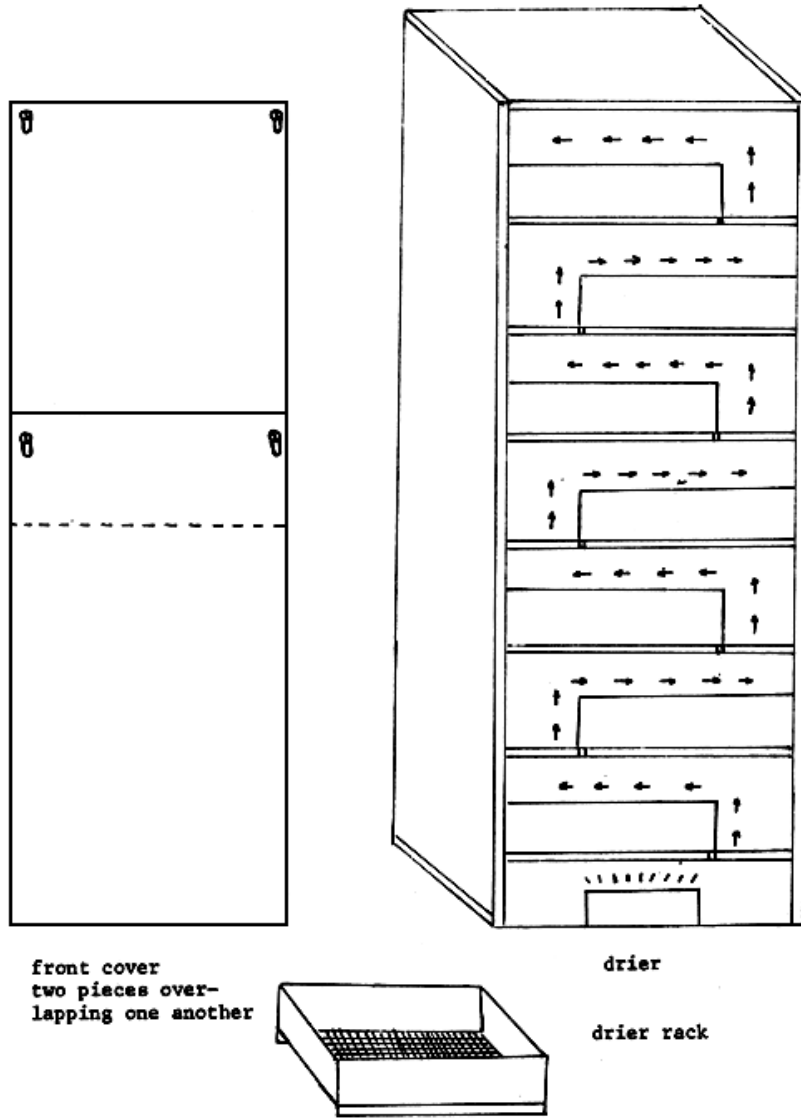
Fig. 8. Improvized drying oven
