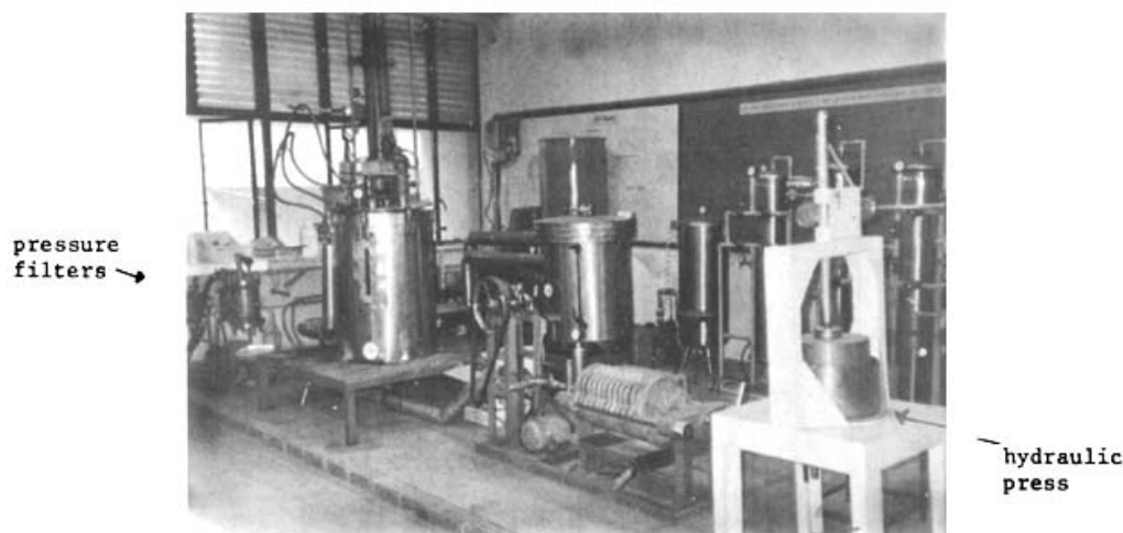
Fig. 12. Prototype agar extraction set-up (capacity - 200 liters)
