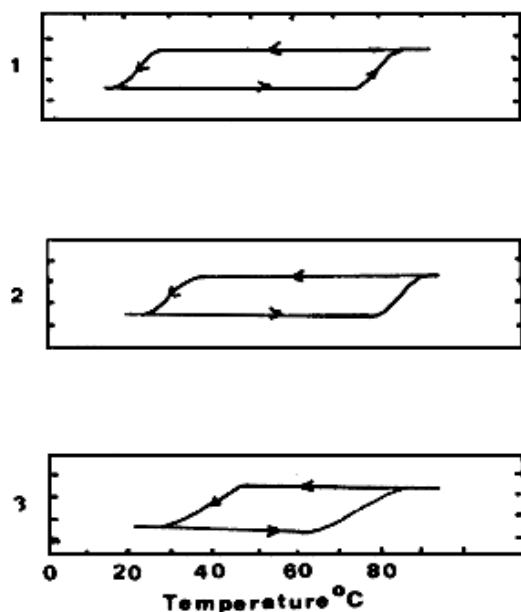
Fig. 3. Changes in optical rotation with the sol-gel transition for agarose samples. 1. Agarose, 2. Agarose with a few 6-O-methyl-D-galactose residues, and 3. Agarose with more 6-O-methyl-D-galactose
