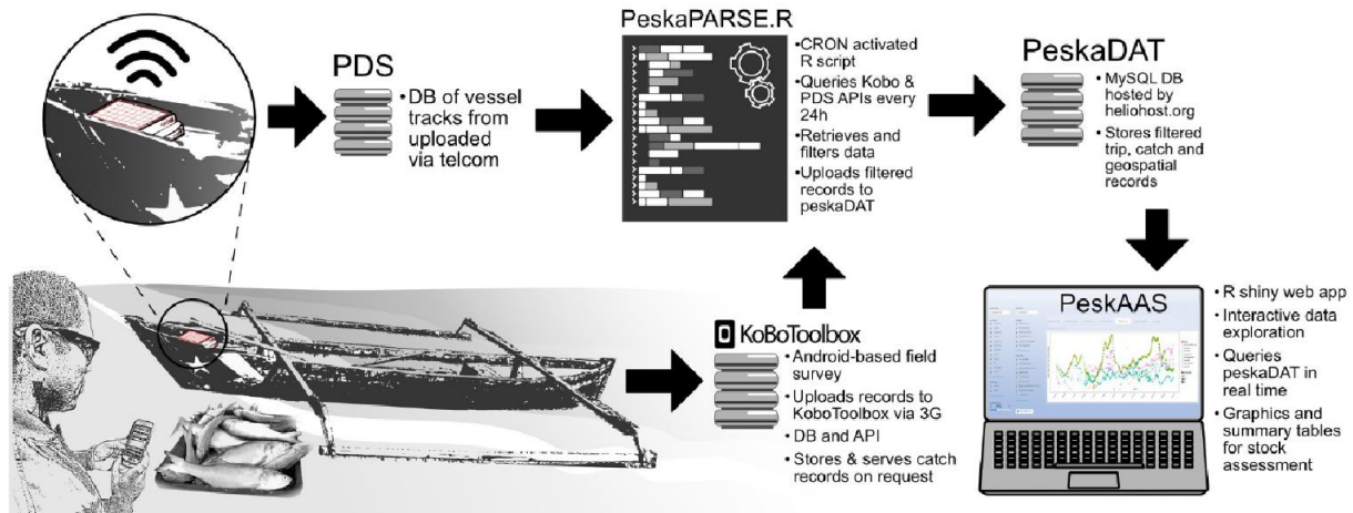
Figure 5. Diagrammatic representation of the PeskaAAS application. From bottom to left, catch data from a vessel are entered into a KoboCollect survey form on a smartphone. These data are uploaded into the KoboToolbox database. An R script (PeskaPARSE.R) pulls brings these data along with the vessel’s movement data obtained by the GPS unit (PDS: Pelagic Data Systems Inc.) in the vessel. These data are then checked and filtered and uploaded into a database (PeskaDAT). The PeskaAAS application can then be used to query the database and provide near-real-time graphics and analytics.
