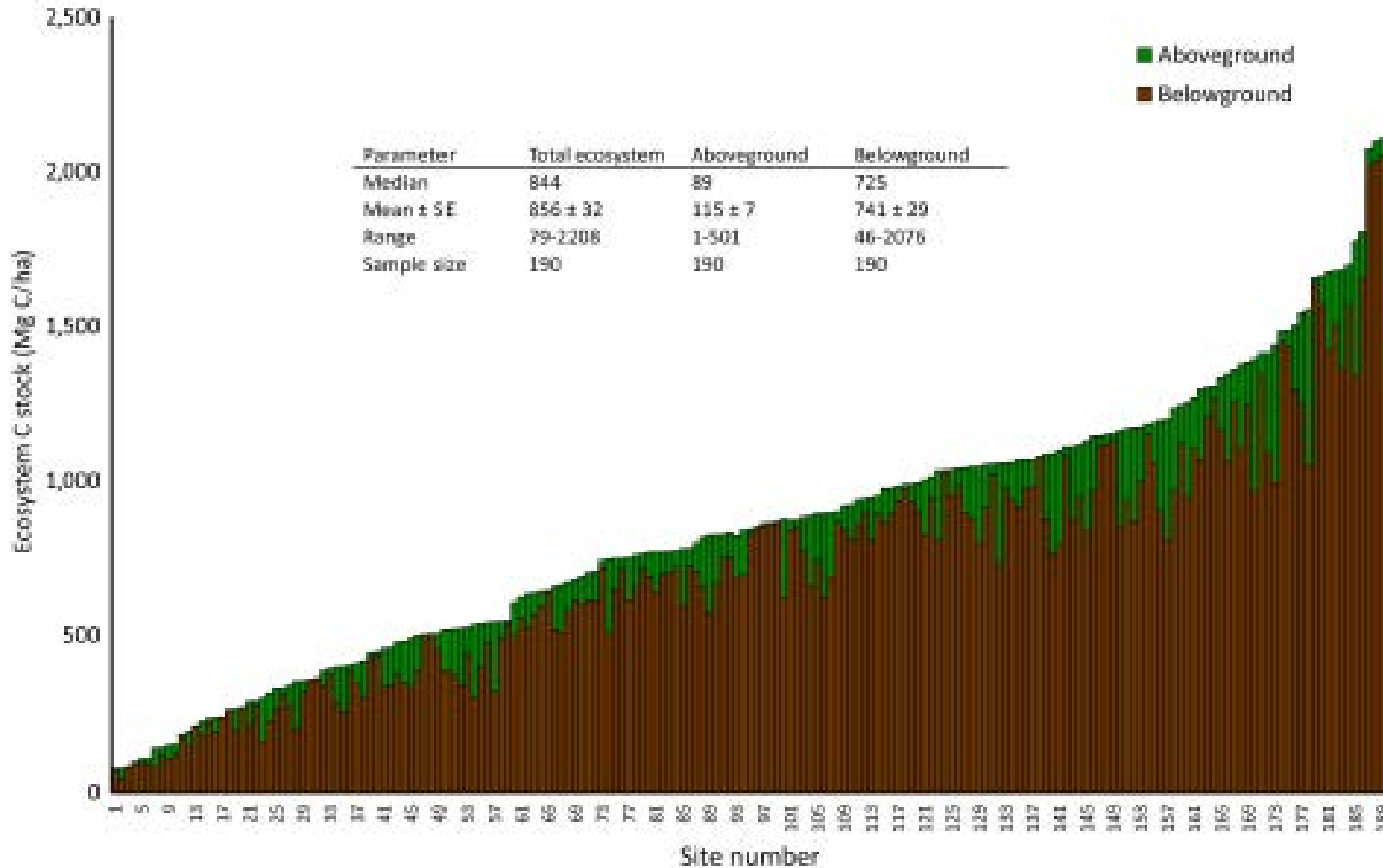
Kauffman et al. Ecol Monog (2020)
