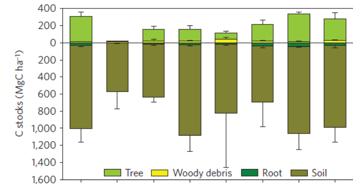
Murdiyarso et al. Nauret Cli Change (2015)
