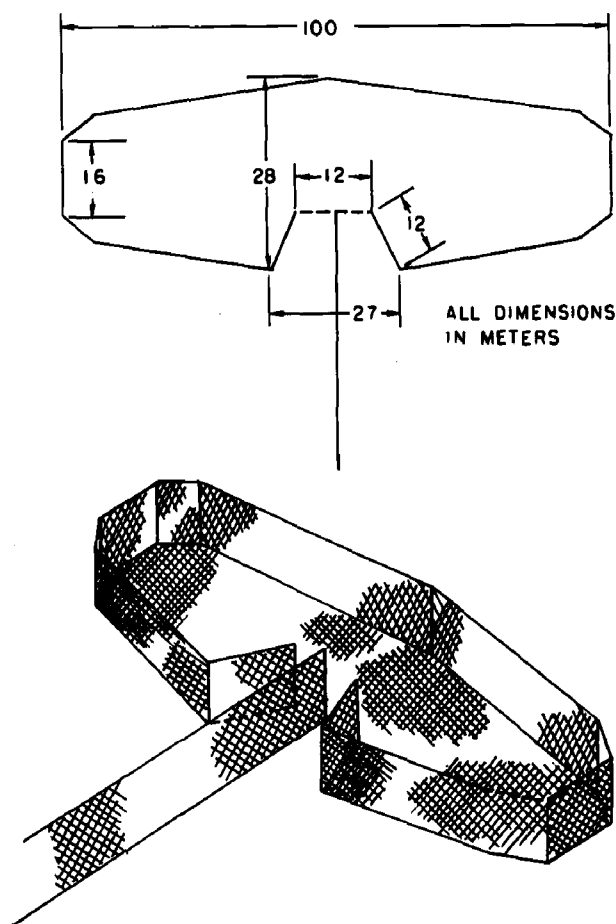
Figure 14.--Plan of Russian salmon trap (Atkinson, 1964).
