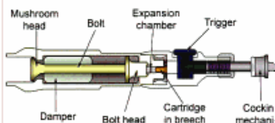
FIGURE 7.7 Non-penetrating CBG with hand trigger (knocker)
