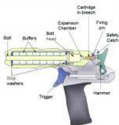
FIGURE 7.5 Penetrating CBG with hand trigger
