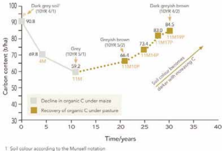
FIGURE 6 Rate of recovery of total C under pasture following intensive cropping
