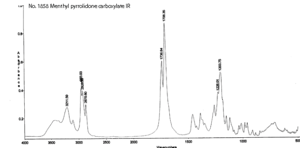
1858 Menthyl pyrrolidone carboxylate (IR)
