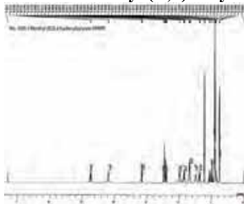
1855 1-Menthyl (R,S)-3-hydroxybutyrate (1H-NMR)
