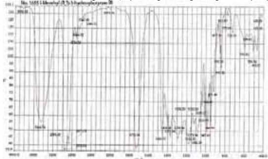
1856 1-Piperitone (1H-NMR)
