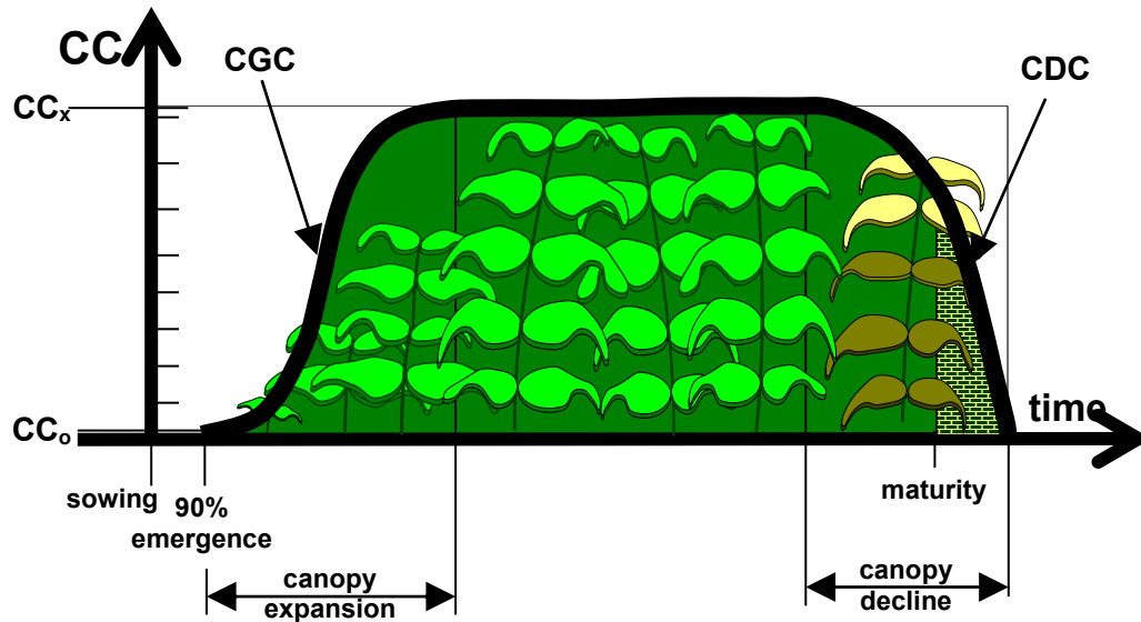
Figure 1.3d – Variation of the green canopy cover (CC) throughout the crop cycle under non-stress conditions. CC_0 and CC_x are the initial and maximum green canopy cover, respectively; CGC is the green canopy growth coefficient; CDC is the green canopy decline coefficient
