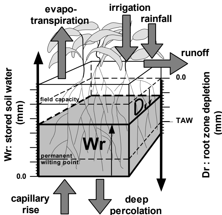
Figure 1.3b – The root zone as a reservoir with indication of the fluxes at its boundaries affecting the water stored in the root zone ( W_r ) and the root zone depletion ( D_r )
