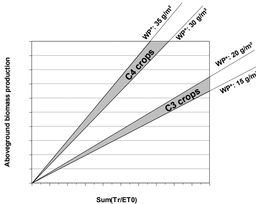
Figure 1.2h – The relationship between the aboveground biomass and total amount of water transpired for C3 and C4 crops after normalization for CO_2 and ET_0 .
