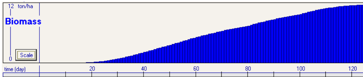
Figure 1.2i – Simulated biomass production throughout the crop cycle for the canopy development and crop transpiration presented in Fig. 1.2g
