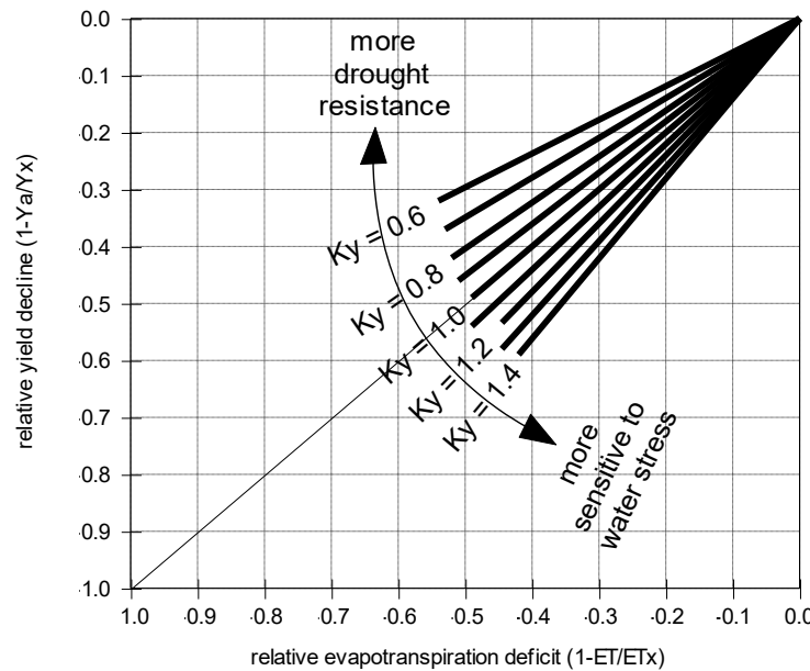
Figure 1.2a – Relationship between relative yield decline (1-Y_a/Y_m) and relative evapotranspiration deficit (1-ET/ET_c) for the total growing period for various values of the seasonal yield response factor ( K_y )
