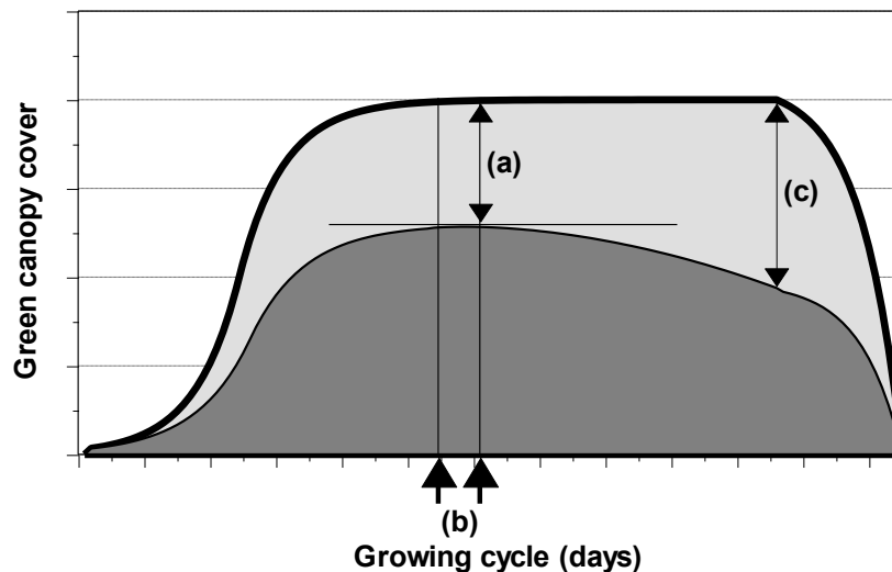
Figure 1.3f – Green canopy cover (CC) for unlimited (light shaded area) and limited (dark shaded area) soil fertility with indication of the processes resulting in (a) a less dense canopy cover, (b) a slower canopy development, and (c) a steady decline of CC once the maximum canopy cover is reached
