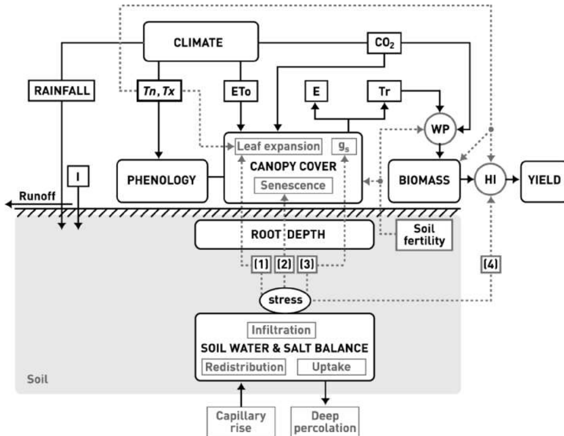
Figure 1.2b – Chart of AquaCrop indicating the main components of the soil–plant–atmosphere continuum and the parameters driving phenology, canopy cover, transpiration, biomass production, and final yield. [I, irrigation; T_n , minimum air temperature; T_x , maximum air temperature; E_{To} , reference evapotranspiration; E , soil evaporation; Tr , canopy transpiration; g_s , stomatal conductance; WP , water productivity; HI , harvest index; CO_2 , atmospheric carbon dioxide concentration; (1), (2), (3), (4), water stress response functions for leaf expansion, senescence, stomatal conductance and harvest index, respectively]. Continuous lines indicate direct links between variables and processes. Dashed lines indicate feedbacks. See section 1.2 for a more extensive description.
