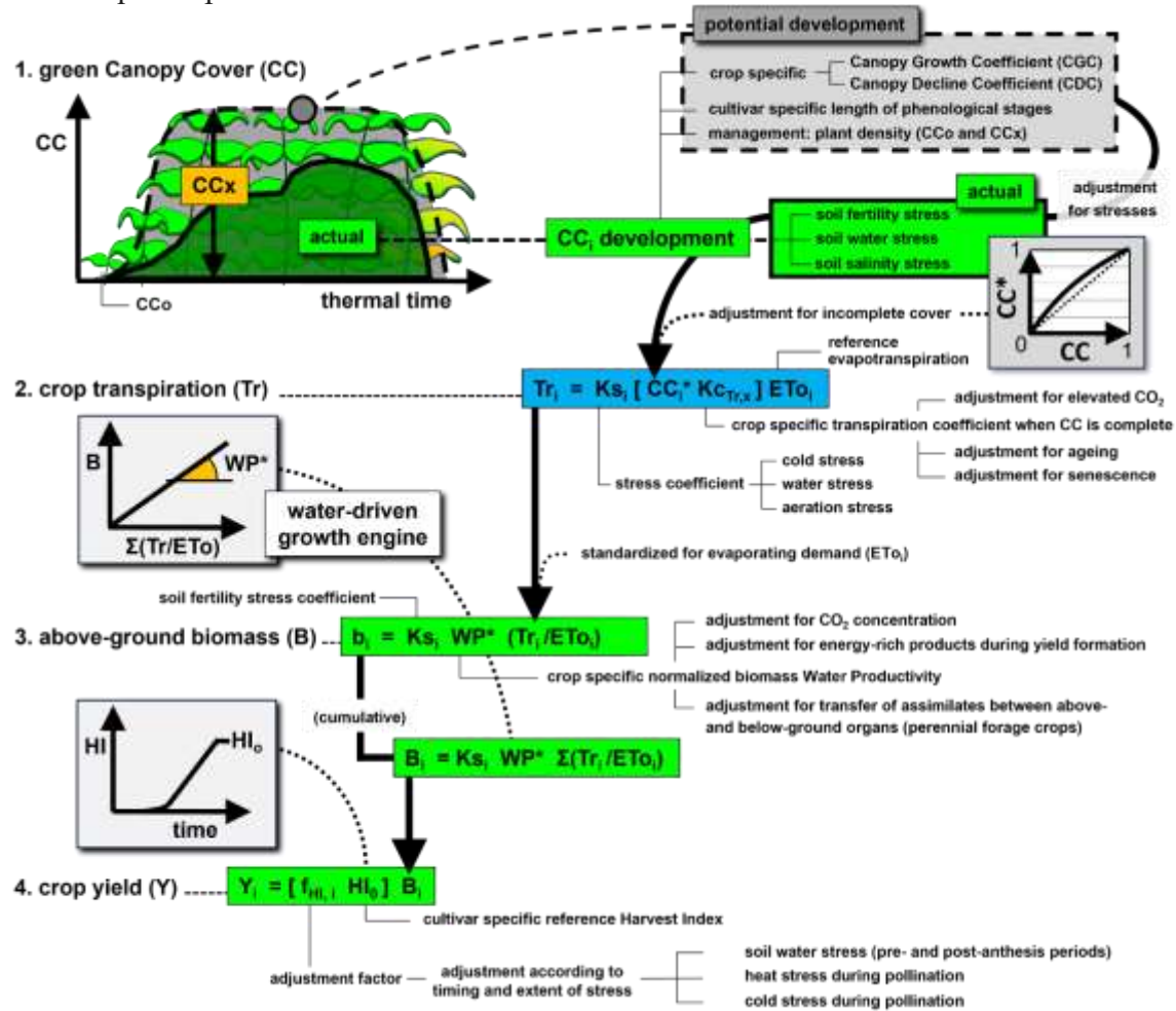
Figure 1.3a –Infographic of the calculation scheme of AquaCrop (Raes et al., 2025).
