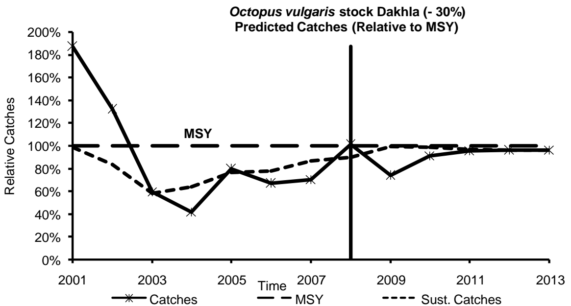
Figure 5.3.5b : Predicted catches and abundance of Octopus vulgaris Dakhla stock – Scenario2 (-30% effort)
