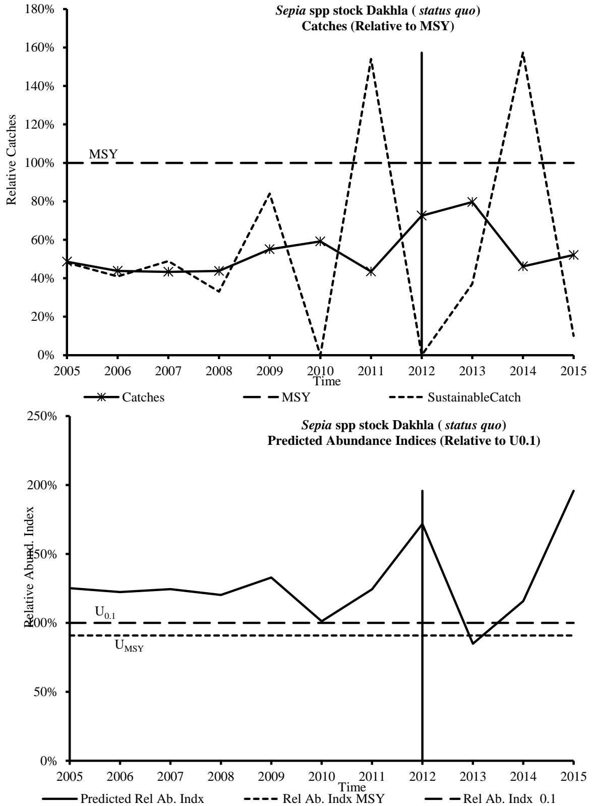
Figure 5.4.5a: Sepia spp. –Dakhla- Projected trends in catches and abundance – Scenario Status quo ) Projection des tendances dans les captures et de l’abondance Scenarior ( Status quo )
