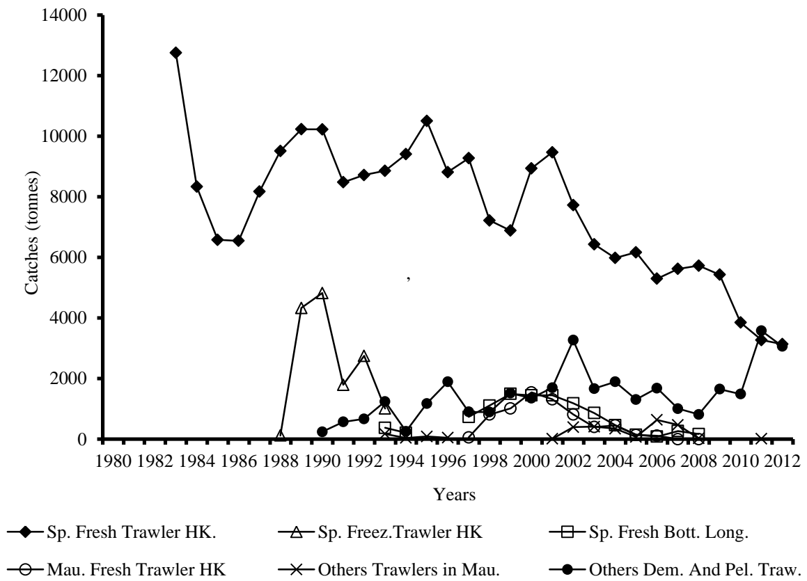
Figure 2.4.3b: Catches (tonnes) of black hake, Merluccius polli and M. senegalensis , in Mauritania Captures (tonnes) de merlu noir, Merluccius polli and M. senegalensis , dans la Mauritanie
