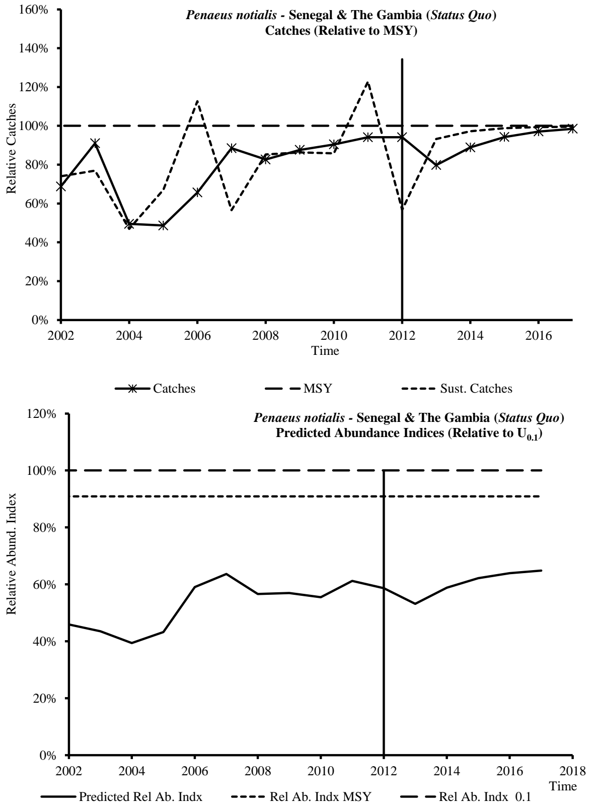
Figure 4.4.5b. P. notialis . Projections of biomass and catches under statu quo scenario (fishing effort maintained at its current level)
