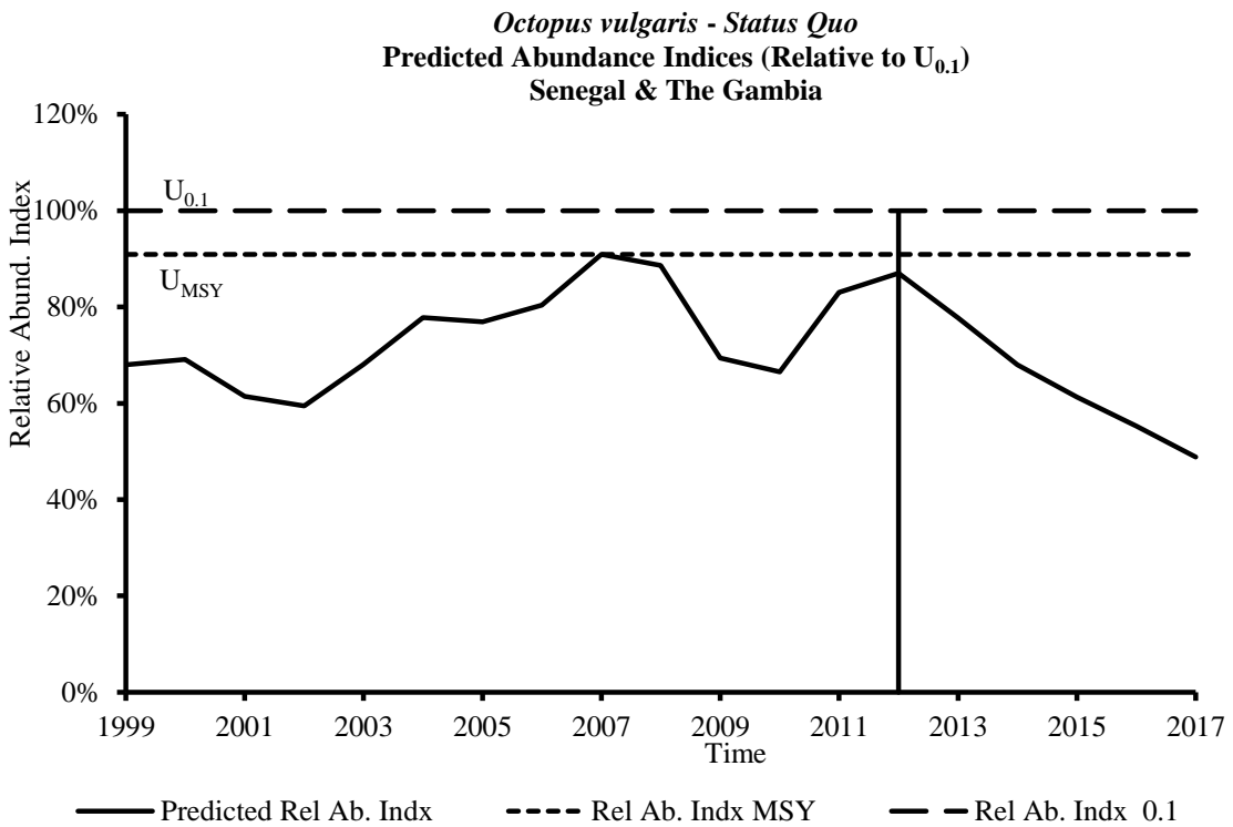
Figure 5.3.5b: Octopus vulgaris –Senegal & The Gambia- Projected trends in catches and abundance – Scenario Status quo Projection des tendances dans les captures et de l'abondance Scenario ( Status quo )
