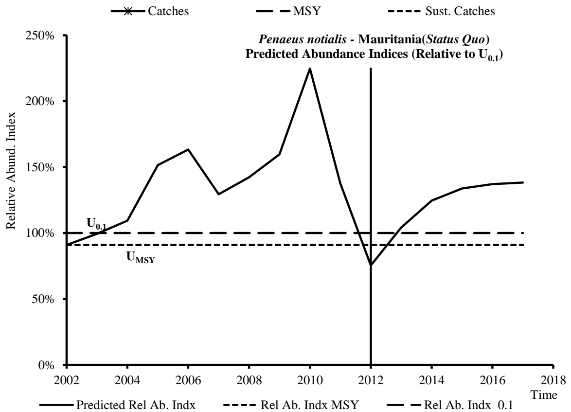
Figure 4.4.5a: P. notialis . Mauritania-Projections of biomass and catches under status quo scenario (fishing effort maintained at its current level) P. notialis .Mauritanie-Projections de la biomasse et des captures selon le scenario de status quo (effort de pêche maintenu à son niveau actuel)
