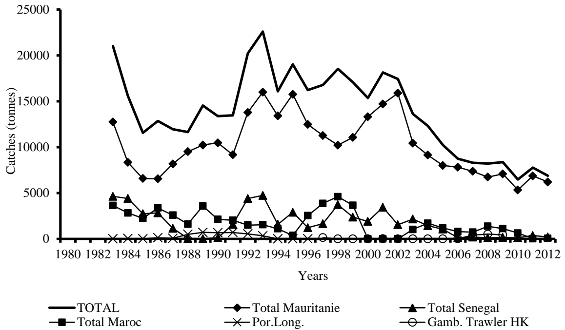
Figure 2.4.3a: Catches (tonnes) of black hake, Merluccius polli and M. senegalensis , in the north of CECAF area Captures (tonnes) de merlu noir, Merluccius polli and M. senegalensis , dans le nord de la zone COPACE
