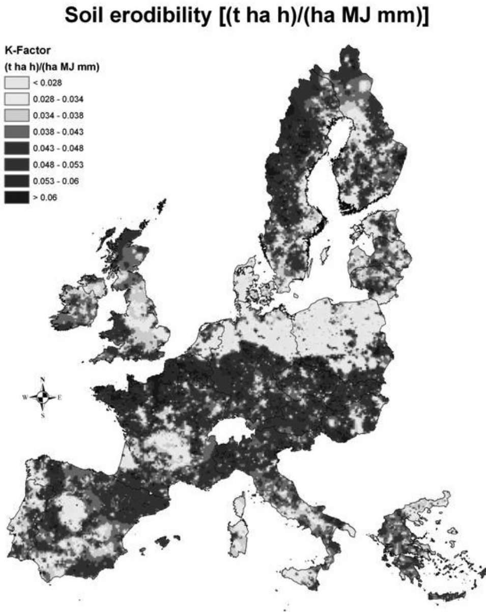
Figure 8. Soil erodibility in Europe
