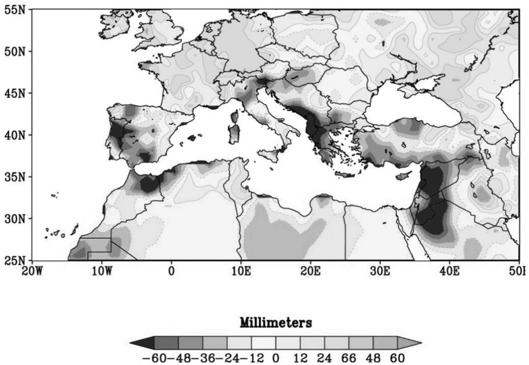
Figure 1. Greyscales highlight lands around the Mediterranean that experienced significantly drier winters during 1971–2010 than the comparison period of 1902–2010
