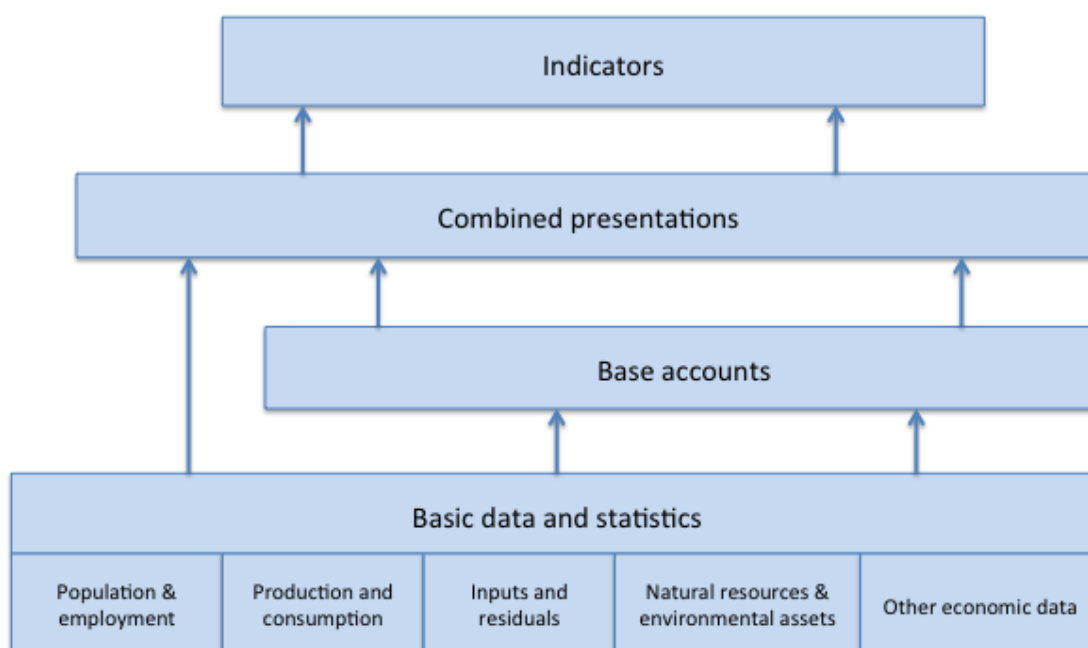
Figure 2.1. SEEA AFF Information Pyramid
