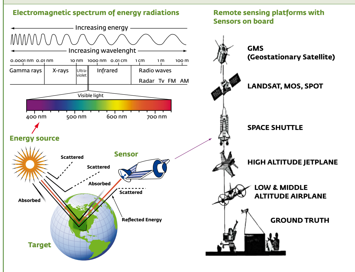
Figure 4.3 Theory of remote sensing of the earth
