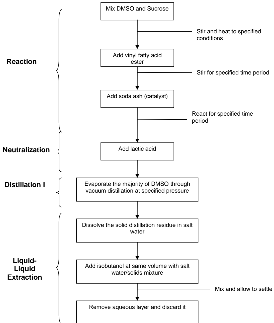
Figure 1. Outline of Manufacturing Process for Sucrose monoesters of lauric, palmitic or stearic acid
