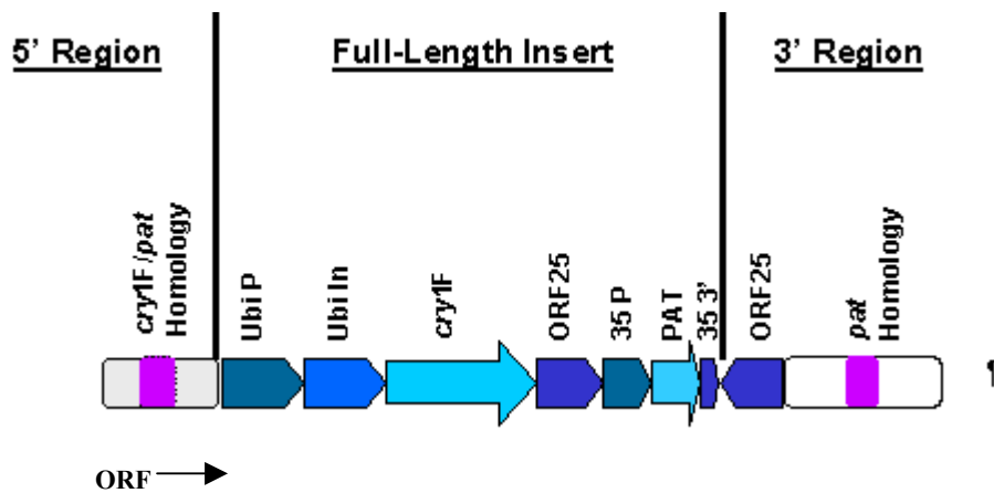
Figure 2. Diagram of inserted genes in corn line 1507
