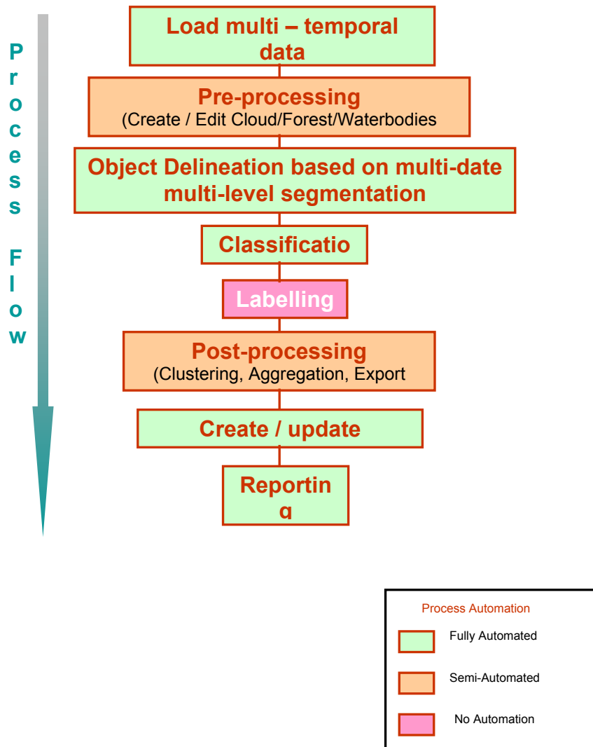
Fig17 - Object-Based process flow
