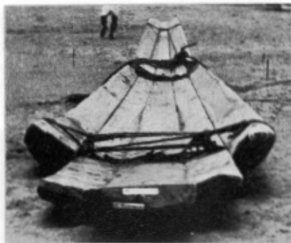
An assembled five-log kattumaram at the Marina in Madras.
