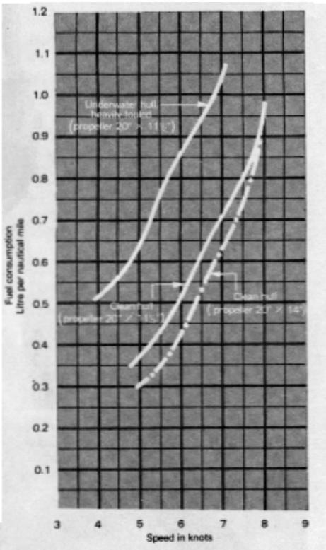
Figure 2 : Fuel consumption per nautical mile. Heavily fouled hull vs. clean hull.
