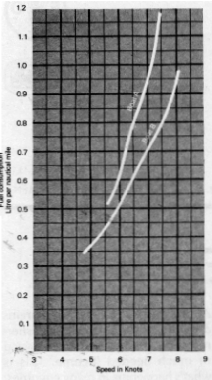
Figure 1 Fuel consumption per nautical mile : Boat A vs. Boat B (both 28-footers)
