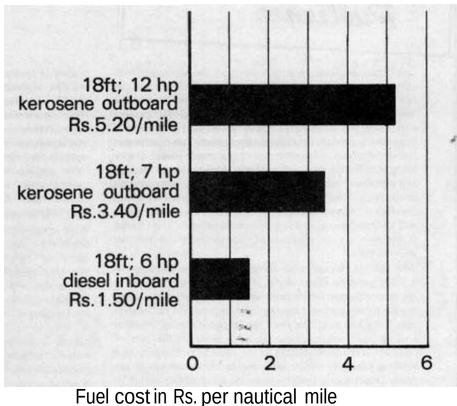
Figure 4 : Fuel cost per nautical mile: Three 18-footers with different engines (12 hp, 7 hp, 6 hp).
