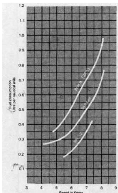
Figure 3 : Fuel consumption per nautical mile : 28-footer vs. 24-footer vs. SRL 12.
