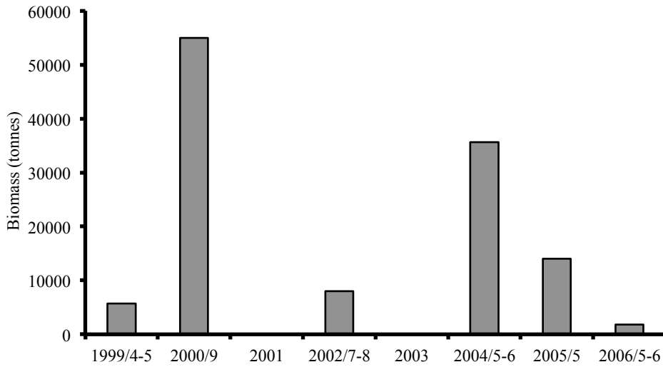
Figure 4.3.2: Biomass estimate of E. encrasicolus (Stock West: Ghana, Togo and Benin) for R/V DR. Fridtjof Nansen /Estimations de la biomasse de E. encrasicolus (Stock ouest: Ghana, Togo et Bénin) pour le N/R Dr Fridtjof Nansen
