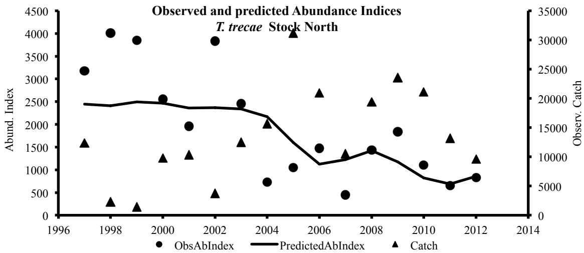
Figure 5.6.1b: Catch (tonnes), predicted and observed abundance indices for T. trecae (Stock North)/Captures (tonnes), indices d'abondance prévus et observés pour T. trecae (stock nord)
