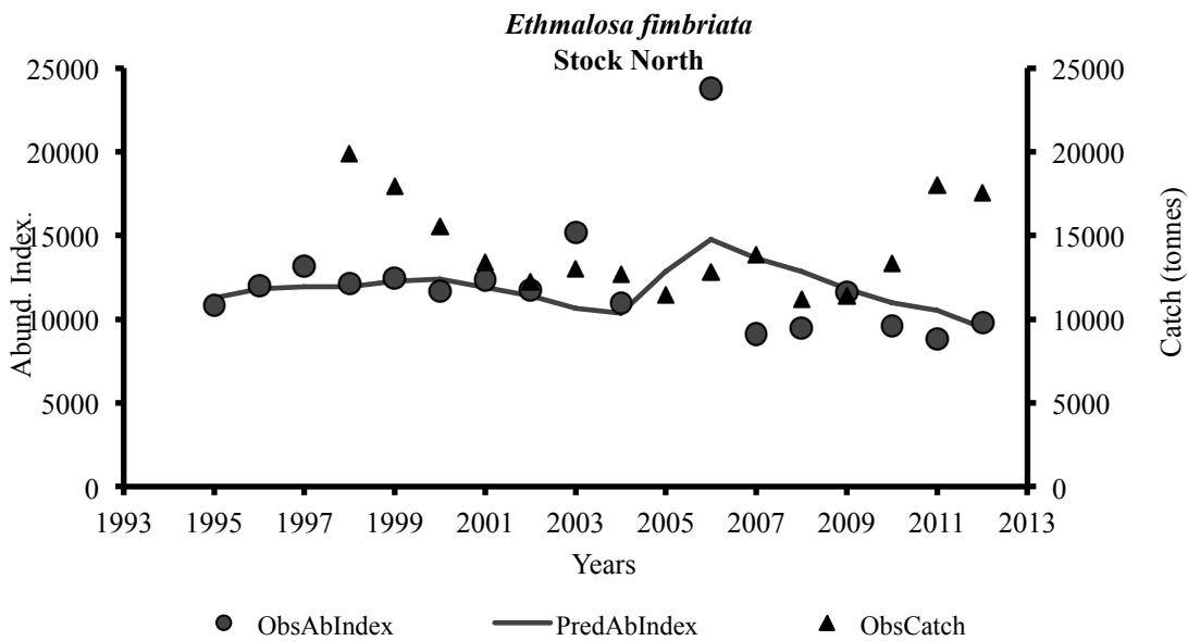
Figure 3.6.1: Catch (tonnes), predicted and observed abundance indices for Ethmalosa fimbriata (Stock North)/Capture (tonnes), indices d'abondance prévus et observés pour Ethmalosa fimbriata (Stock nord)
