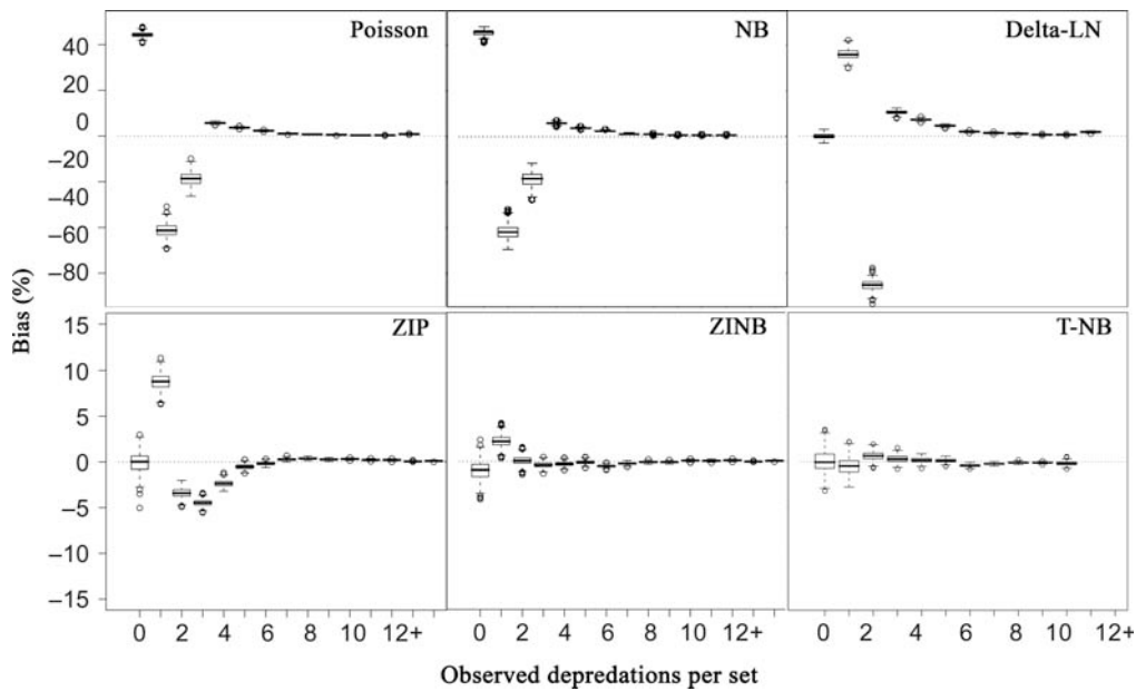
Figure 3. Relative bias plots between observed and predicted deprecations from the best-fitting Poisson, negative binomial (NB), Delta-LN, ZIP, ZINB, and T-NB models, based on 300 resamples of the US pelagic longline observer dataset. For each iteration, model parameters estimated from half the dataset were used to predict the remaining observations, with bias calculated as the discrepancy between predicted and observed values.
