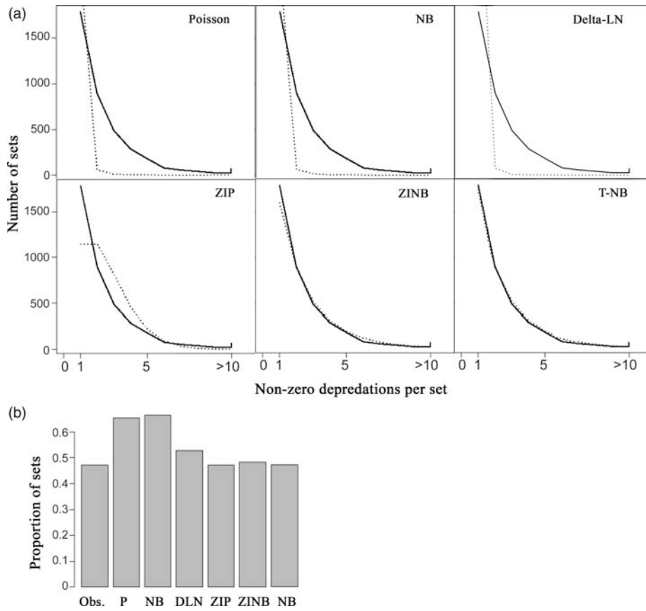
Figure 2. Observed and predicted frequencies of depredation events per set in the US Atlantic pelagic longline fishery. Plots include frequencies of (a) positive counts and (b) zeroes.
