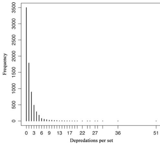
Figure 1. Observed frequency distribution for depredations per set in the US Atlantic pelagic longline fishery, 1992–2006.
