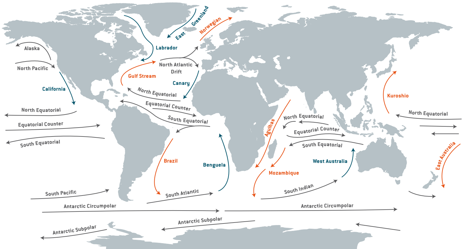
OCEAN CURRENTS
