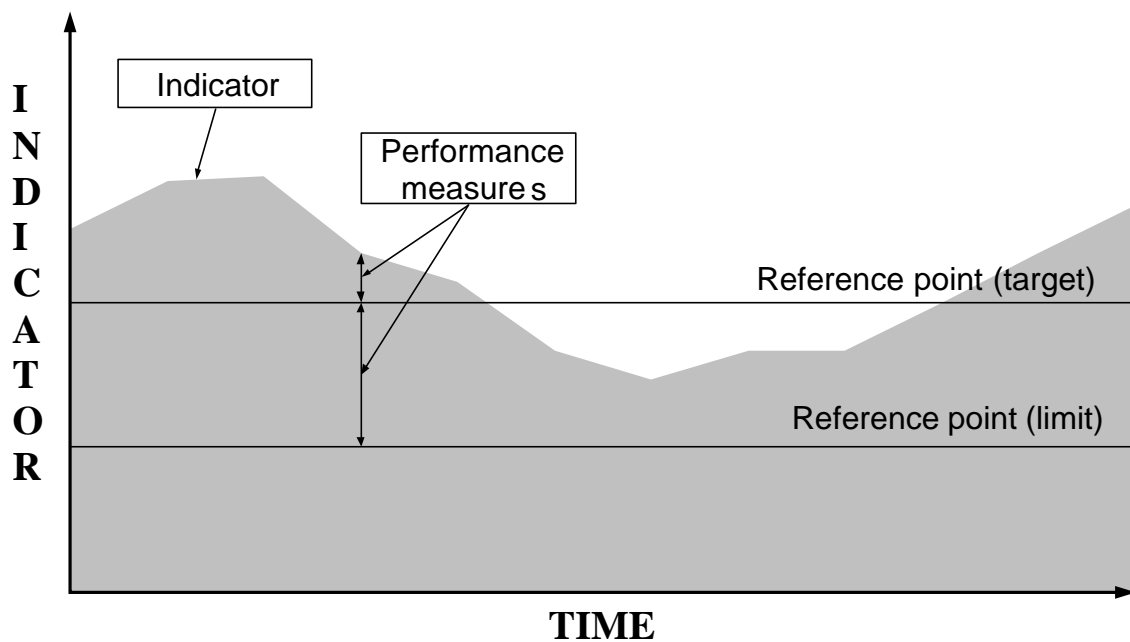
Figure 3. The use of an indicator and reference points to define simple performance measures, the difference between the indicator variable and its target or limit reference point in any year.
