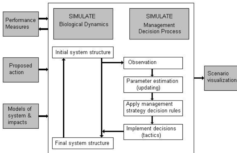
Figure 2. Framework for Management Strategy Evaluation (MSE). Performance measures are derived from management objectives and would at least include measures relating to ecological and fishery production. The biological dynamics are simulated using a model or a series of models that represent knowledge and uncertainty about the way the biological world works. Prospective management strategies are simulated as they interact with the biological model. A strategy includes the observations (monitoring) made, the analysis of those observations to update management related parameters, use of these updated parameters in management decision-making, and implementation of decisions. Alternative management strategies can be compared using the common currency of the chosen performance measures. From Sainsbury et al. , 2000.
