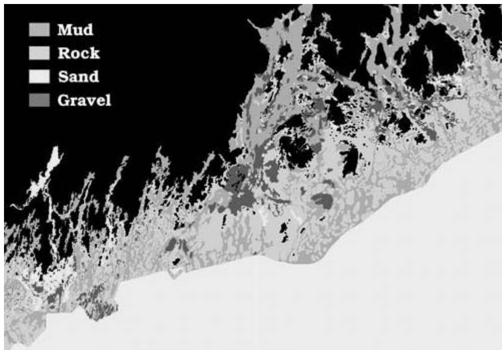
Figure 5. Map of surficial geology as captured by side scan sonar, and interpreted using GIS layers that describe the spatial distribution of rock, sand, gravel and mud on the sea floor. Source: Mapping Penobscot Bay: Surficial Geology, by Joe Kelly, University of Maine (see www.penbay.net/geology.htm )
