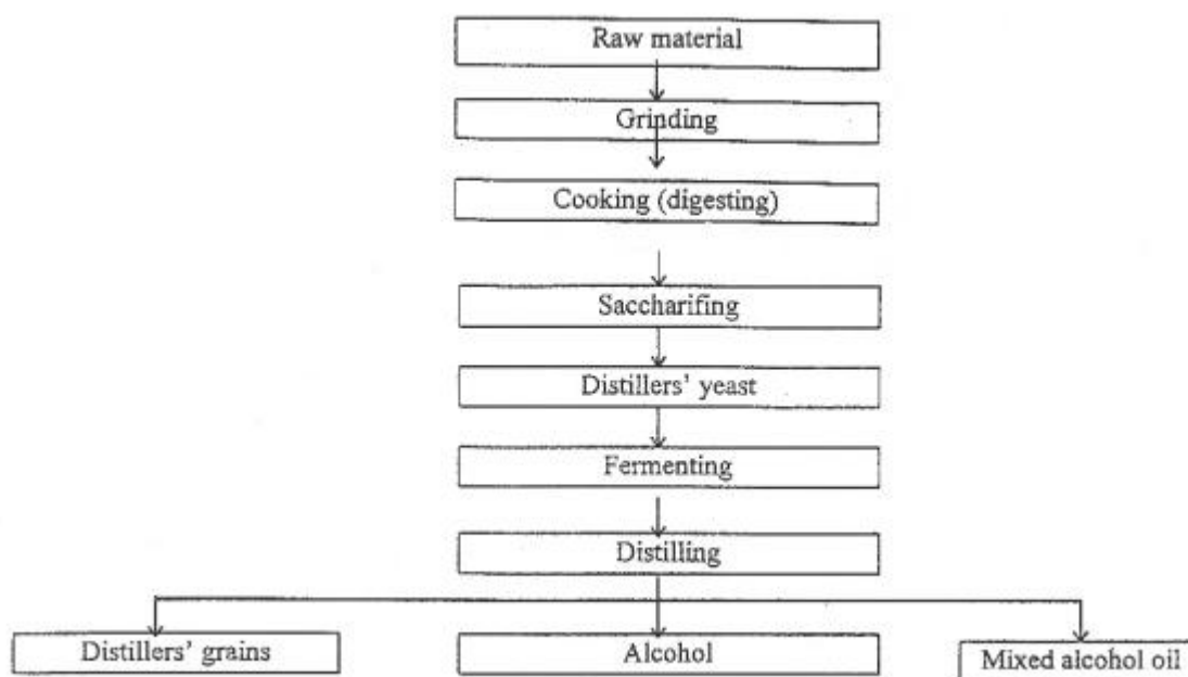
Figure 12: Flow Figure of Making Alcohol
