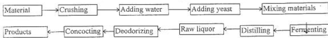
Figure 5: Processing Method of Liquor Using Sweet Sorghum Stalk
