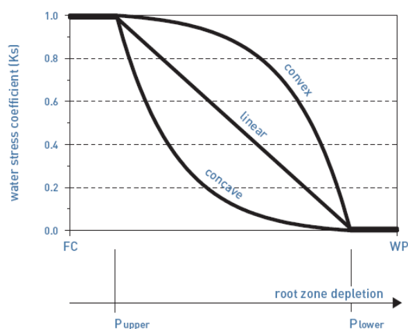
Fig. 3. Examples of K_s response function to the relative depletion in soil water content. The function assumes linear shape when f_{shape}=1 , concave shape when f_{shape}<0 , and convex shape when f_{shape}>0 .
