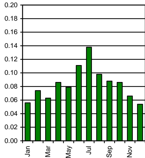
Figure 6: Temporal distribution of BQ in AP (proportion of outbreaks by month)
