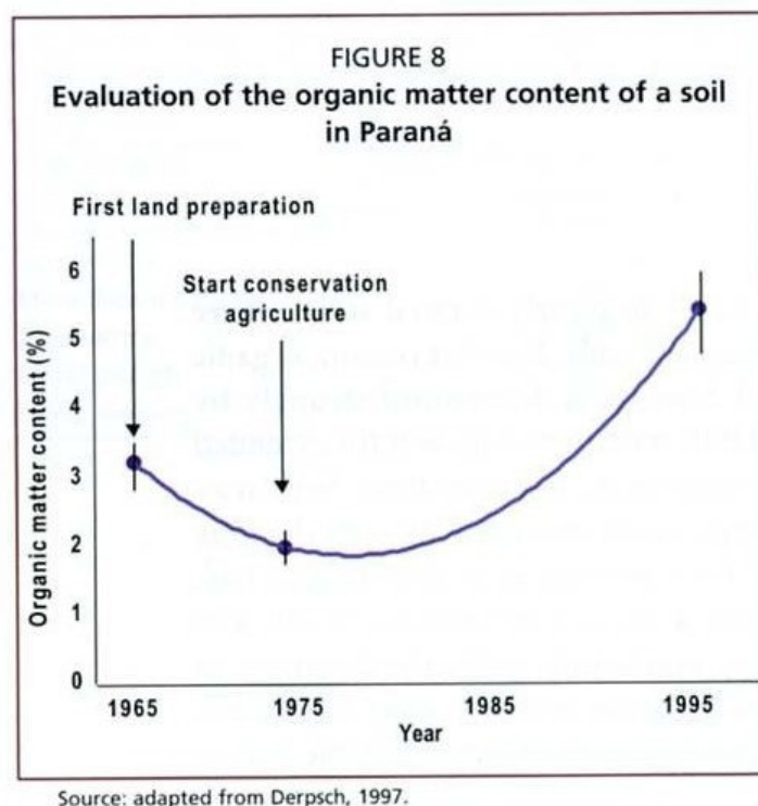
Figure 5: Reversal of s.o.m. decline by adoption of CA in Paraná, Brazil. Source: Bot A., Benites J., 2005: 'The Importance of Soil Organic Matter'. FAO Soils Bulletin 80, p.20.
